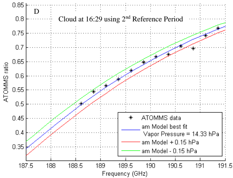
Figure 5: Examples of fitting the observed ATOMMS amplitude ratio, Eq. (2) (black asterisks), to the forward calculated ATOMMS ratio using using am7.2 . Blue line is the best fit line for the indicated vapor pressure. Red line is am forward calculation for a vapor pressure 0.15 hPa greater than the best fit vapor pressure. Green line is forward calculation for a vapor pressure 0.15 hPa less than the best fit vapor pressure. The solutions shown in panels A, B, and C used reference period 1, while the solution in panel D used reference period 2.
