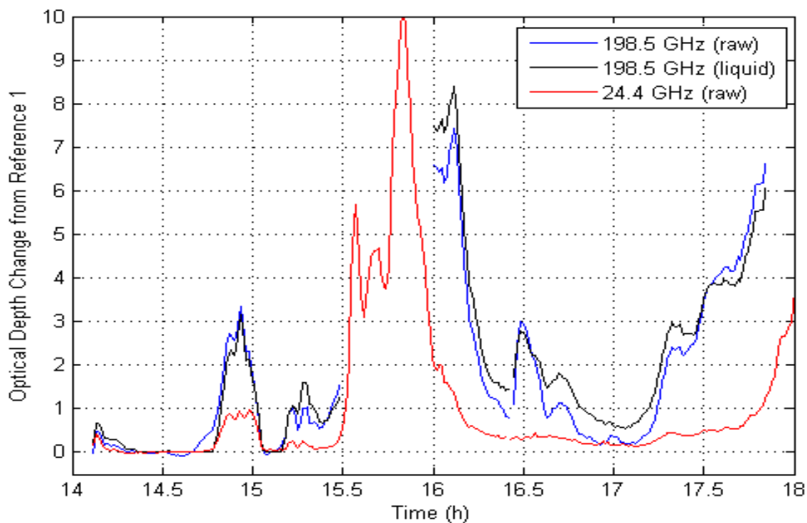
5 Figure 2: Blue and red lines show observed changes in optical depth at 198.5 GHz and 24.4 GHz relative to reference period 1. The black line shows changes in optical depth at 198.5 GHz due to changes in liquid water after removing the contribution from changes in vapor pressure and temperature.
