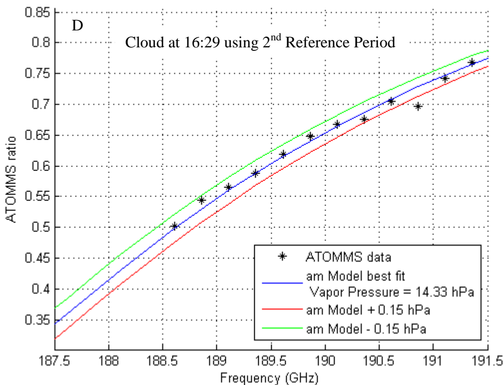
5 Figure 5: Examples of fitting the observed ATOMMS amplitude ratio, Eq. (2) (black asterisks), to the forward calculated ATOMMS ratio using the am Model, version 7.2. Blue line is the best fit line for the indicated vapor pressure. Red line is am forward calculation for a vapor pressure 0.15 hPa greater than the best fit vapor pressure. Green line is forward calculation for a vapor pressure 0.15 hPa less than the best fit vapor pressure. The solutions shown in panels A, B, and C used reference period 1, while the solution in panel D used reference period 2.
