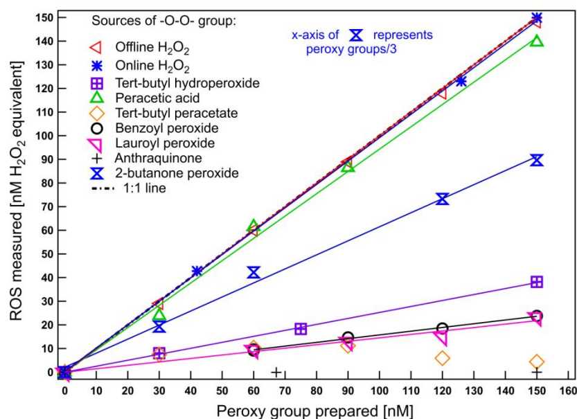
Figure 3. Calibration curves of H 2 O 2 and response of selected compounds. Linear fits are shown for different peroxides and other compounds of interest in the concentration range of 0 to 150 nM. The correlation coefficients R^2 were 0.99, except for lauroyl peroxide ( R^2 = 0.91 ).
