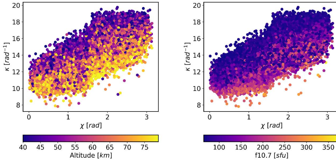
Figure 11. \kappa vs. solar zenith angle ( \chi ), colour coded by altitude (left) and f10.7 (right).
