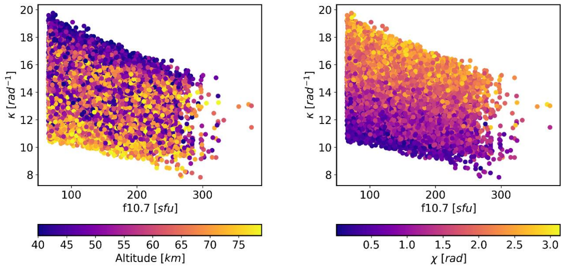
5 Figure 12. \kappa vs. f10.7, colour coded by altitude (left) and solar zenith angle ( \chi ) (right)
