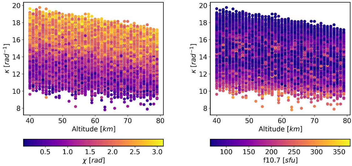
Figure 13. \kappa vs. altitude, colour coded by solar zenith angle ( \chi ) (left) and f10.7 (right)
