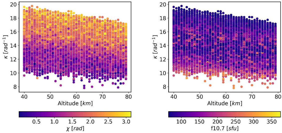
Figure 13. \kappa vs. altitude, colour coded by solar zenith angle ( \chi ) (left) and f10.7 (right). 1 sfu = 10^{-22} Wm -2 Hz -1
