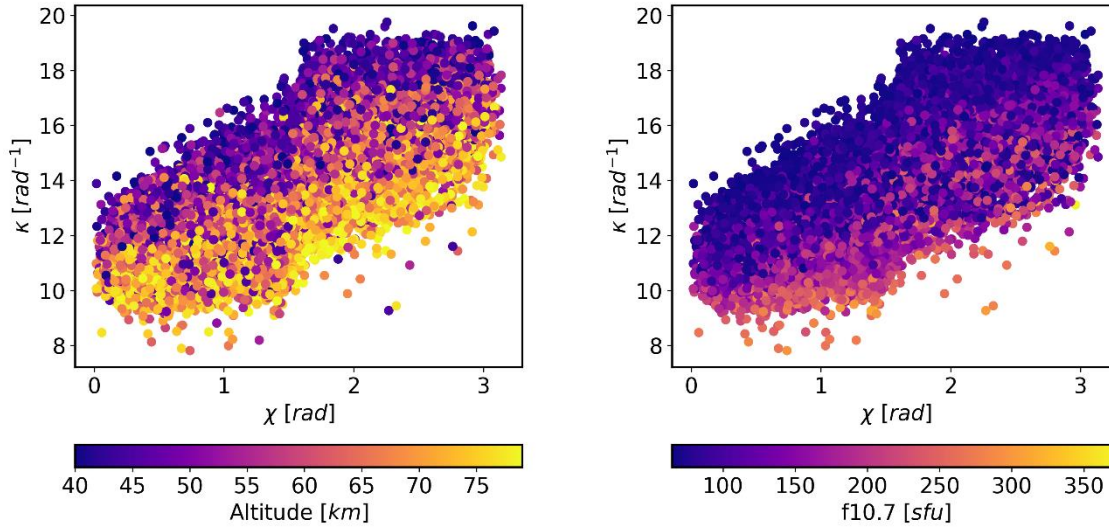
Figure 11. \kappa vs. solar zenith angle ( \chi ), colour coded by altitude (left) and f10.7 (right). 1 sfu = 10^{-22} Wm -2 Hz -1
