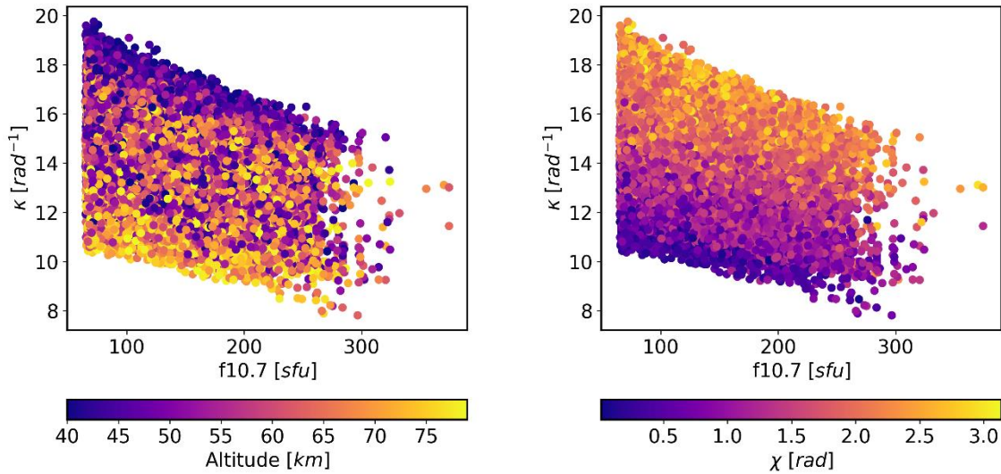
5 Figure 12. \kappa vs. f10.7, colour coded by altitude (left) and solar zenith angle ( \chi ) (right). 1 sfu = 10^{-22} Wm -2 Hz -1
