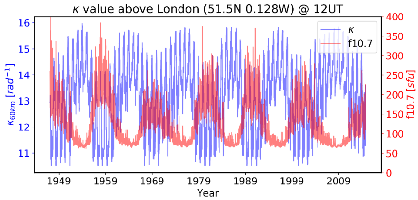
Figure 9. Solar cycle dependence of \kappa for a fixed location (London), tangent height (60 km) and local time (12UT). 1 \text{ sfu} = 10^{-22} \text{ Wm}^{-2}\text{Hz}^{-1}
