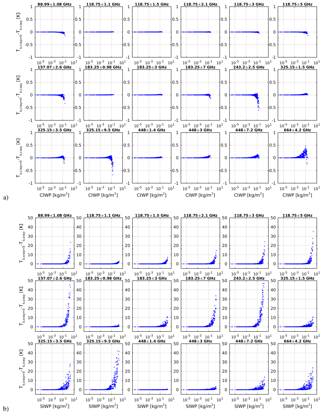
Figure 2. Difference in brightness temperatures between simulations with (a) cloud ice set to zero and with simulation with unchanged cloud ice as a function of the CIWP, (b) same as for (a) but with snow set to zero and as a function of SIWP.
