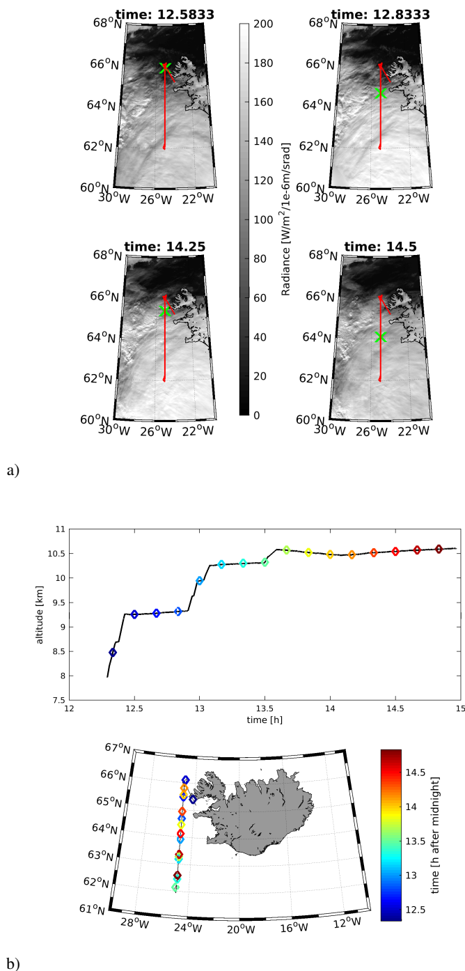
Figure 5. (a) Images of MODIS (Terra and Aqua) band 1 (visible) during flight B897 on March 18, 2015 overlaid with the flight track (red lines) and the position of the aircraft (green crosses) at the MODIS measurement time. (b) Altitude time series of flight B897 and below map with the flight track (black) with a color marker indicating the time.
