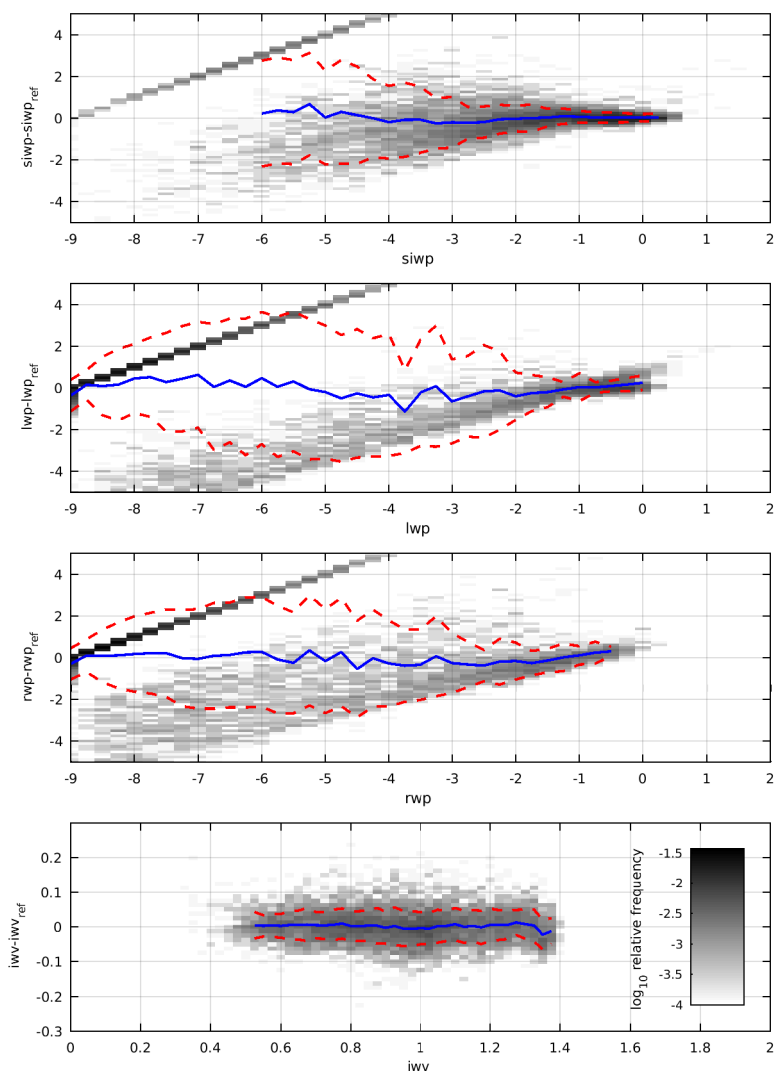
Figure 3. Two-dimensional histograms of the difference between components of the retrieved state vector and the corresponding ICON model state vector, as a function of the retrieved state vector. The components of the state vectors are defined as the decadal logarithm of the ratio of the specific quantity and the specific unit path, therefore they are unitless. The offsets O of the components of the retrieved state vector are shown as blue lines and the corresponding standard deviations \sigma_O are shown as red lines. For the hydrometeor paths, an x-value of -3 corresponds to a value of 10^{-3} \text{ kg/m}^2 = 1 \text{ g/m}^2 . For IWV, an x-value of 1 corresponds to a value of 10^1 \text{ kg/m}^2 = 10 \text{ kg/m}^2 .
