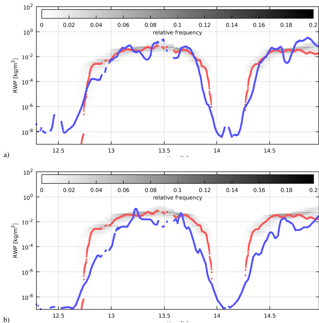
Figure 8. (a) Time series of the retrieved RWP. The time series of the retrieved RWP is shown as a blue line. The time series of the ICON model RWP for the time and location of the FAAM during flight B897 is shown as red line. Time series of histograms of the ICON model RWP are plotted as grey shades underneath, see text for details. (b) The same as in the top figure, but the RWP retrieved from the simulated flight.
