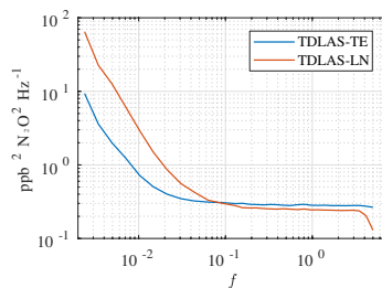
Figure 7: Mean \text{N}_2\text{O} variance spectra of each TDLAS analyzer from 29 June 2016 to 9 July 2016.
