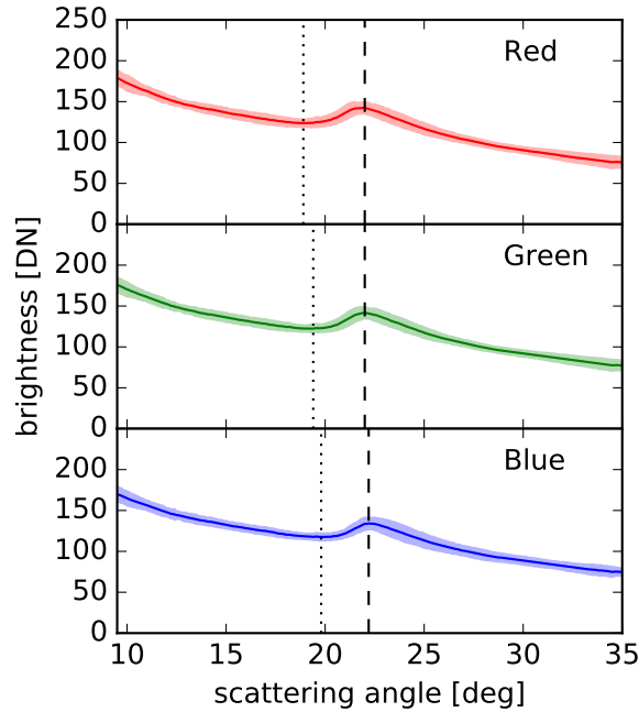
Figure 5. HaloCam image processing demonstrated for the same-image-as-measurements shown in Fig. 4, segment no. 4. The three panels show the brightness distributions (in digital numbers [DN]) for the red, green and blue image channel as a function of the scattering angle. The solid line represents the brightness averaged azimuthally over the image segment, whereas the shading indicates the 2\sigma standard deviation. The vertical lines pinpoint the scattering angles of the 22^\circ halo minimum (dotted) and maximum (dashed) for the RGB channels.
