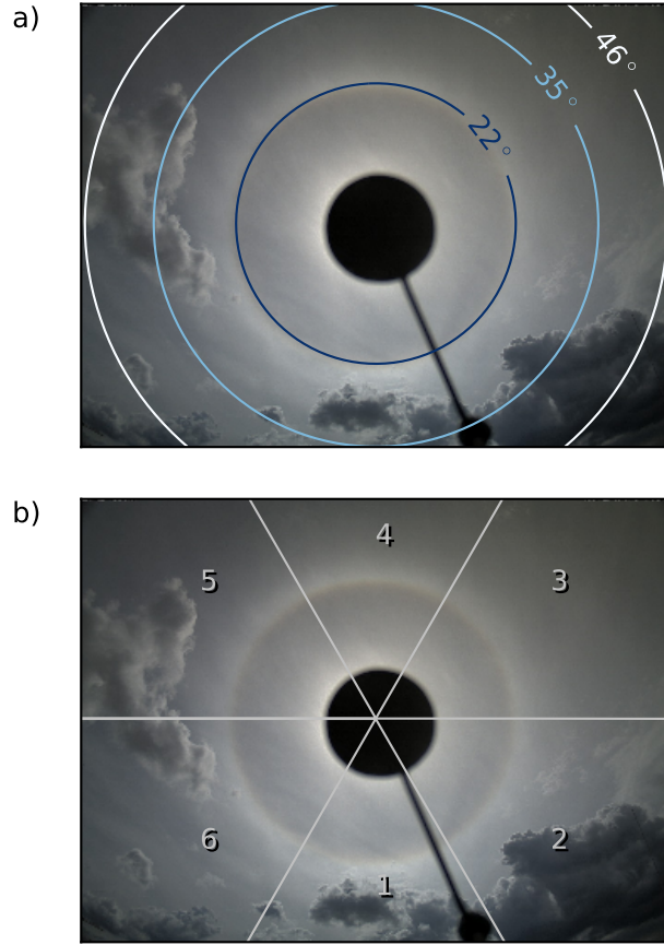
Figure 4. a) HaloCam image from 2014-05-12, 13:52 UTC with corresponding zenith - scattering angle ( \vartheta ) grid and representative contour lines at 22°, 35° and 46°, b) shows the relative azimuth ( \varphi ) grid with numbered labels for the 6 image segments.
