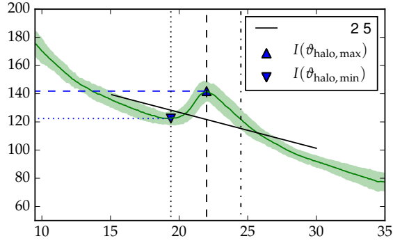
Figure 7. As Fig. 5, but showing \vartheta_{\text{halo,end}} (dash-dot line) in addition to the first minimum (dotted) and the maximum (dashed) of the 22^\circ halo for the green channel. In addition, \vartheta_{\text{halo,end}} is indicated (dash-dot line) which represents the scattering angle of the same brightness as \vartheta_{\text{halo,min}} and confines the halo peak. In this example \vartheta_{\text{halo,end}} is located at about 24.5^\circ . The corresponding brightness I(\vartheta_{\text{halo,min}}) and I(\vartheta_{\text{halo,max}}) used to calculate the HR are marked with the blue triangles pointing down (min) and up (max). The regression line of the averaged brightness distribution (solid black), which is evaluated between scattering angles of 15^\circ and 30^\circ , has a slope of -2.5 for this example.
