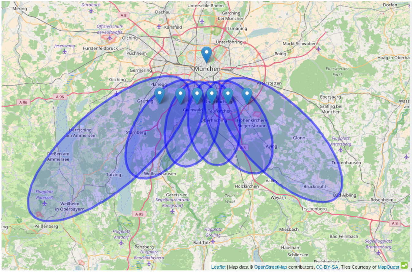
Figure 3. The blue ellipses represent the 22^\circ halo projected on a cirrus cloud deck at 9 km altitude for different solar positions on 21 March between 9 UTC and 13 UTC in 1 h intervals. The blue pins in the focal point of each ellipse indicates the projected position of the sun. The blue pin a bit north of the center of Munich represents the location of the HaloCam site.
