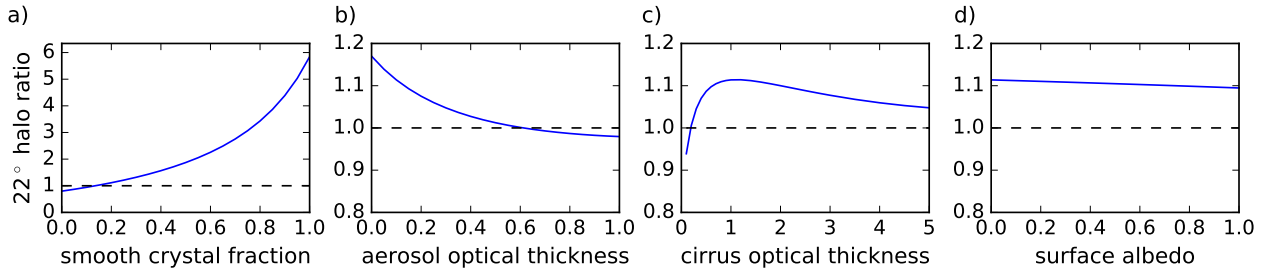
Figure 11. Sensitivity studies of the 22° halo ratio at 550 nm (as defined in Eq. 1) as a function of rough smooth crystal fraction, aerosol optical thickness (AOT), cirrus optical thickness (COT), and surface albedo (from left to right). The radiative transfer simulations were performed with libRadtran assuming an ice cloud between 10 – 11 km using ice crystal optical properties as in Fig. 10 for a solar zenith angle of 60°. The dashed line indicates HR = 1, which marks the threshold for the visibility of a halo display. The default parameters, i.e. if not varied, are 20% smooth solid columns, AOT = 0.2, COT = 1.0, and albedo = 0.0.
