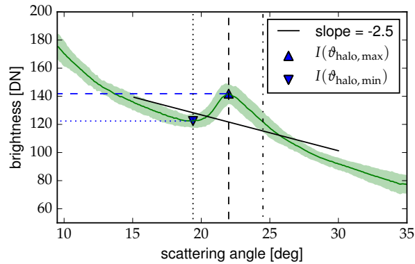
Figure 2. As Fig. 5 showing the first minimum (dotted) and the maximum (dashed) of the 22^\circ halo for the green channel. In addition, \vartheta_{\text{halo, end}} is indicated (dash-dot line) which represents the scattering angle of the same brightness as \vartheta_{\text{halo, min}} and confines the halo peak. In this example \vartheta_{\text{halo, end}} is located at about 24.5^\circ . The corresponding brightness I(\vartheta_{\text{halo, min}}) and I(\vartheta_{\text{halo, max}}) used to calculate the HR are marked with the blue triangles pointing down (min) and up (max). The regression line of the averaged brightness distribution (solid black), which is evaluated between scattering angles of 15^\circ and 30^\circ , has a slope of -2.5 for this example.
