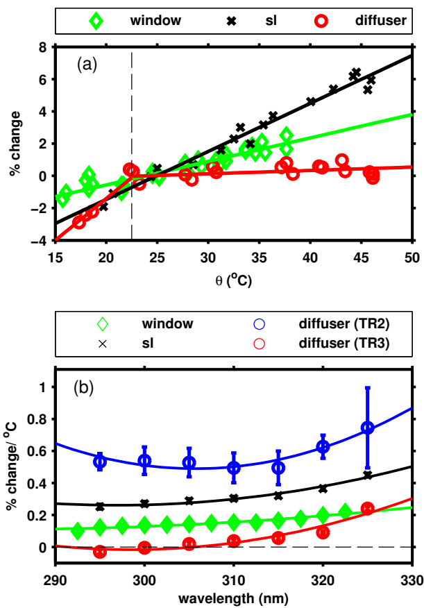
Figure 5. (a) Change in the response of B005 as a function of temperature for the sl and measurements through the window and the diffuser, relative to the response at 25°C and (b) the dependence of the derived slopes from wavelength.
