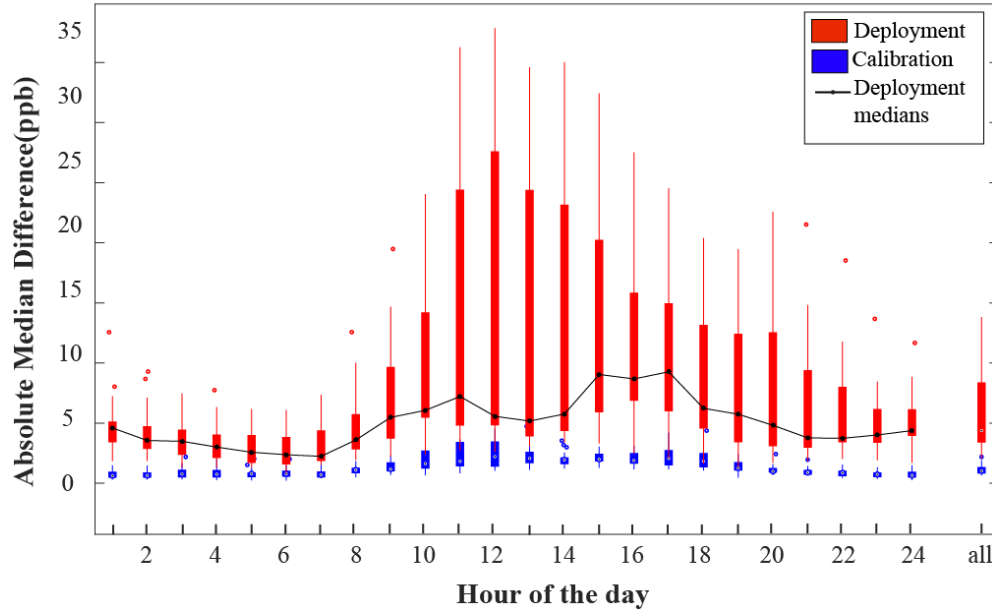
Figure 9. Distributions of medians of absolute differences between all pairs of pods for each hour of the day. Whiskers show 95% intervals. The black line connects the medians of the deployment. The “all” category includes all hours of the day.
