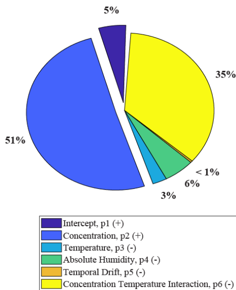
Figure 4: Average relative effect size of model parameters predicting sensor signal ( R/R_o ) from standardized regression coefficients.
