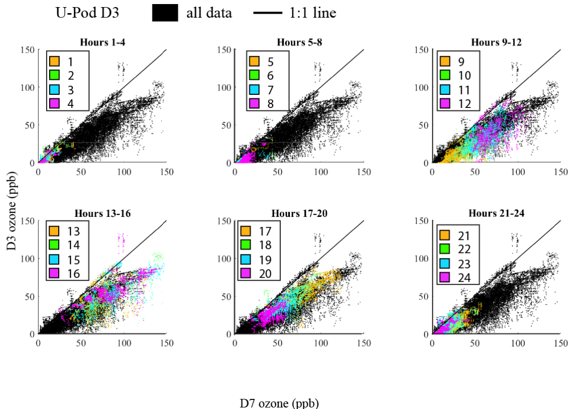
Figure 11. Data from D3, at Industrial Zone 1, plotted against D7 (at Rubidoux). In each scatterplot, colored data in the legend represents four hours of the day, and the black data represents the complete deployment dataset (all hours). The black line is a 1:1 line, not a line of best fit.
