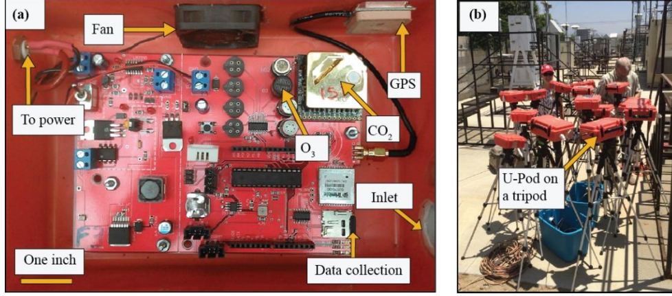
5 Figure 2. Demonstration of the U-Pod layout (a), including sensor locations and other features. (b) A photo of the field calibration collocation at Rubidoux AQMS.
