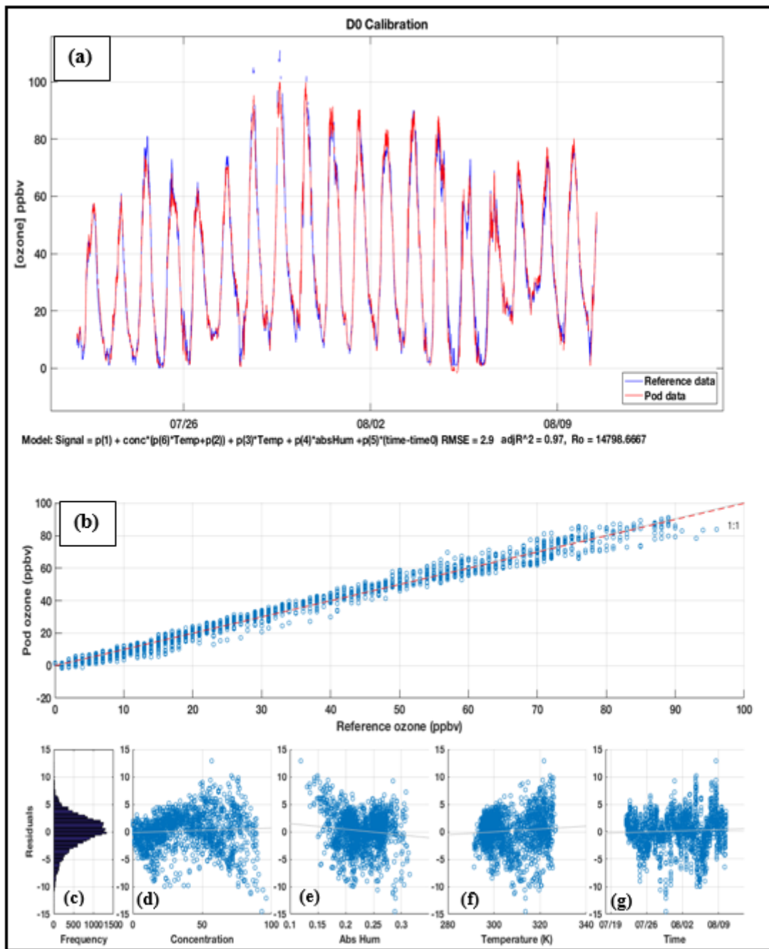
Figure 3. Example calibration results for one ozone sensor in U-Pod D0. Panel (a) shows the modeled ozone sensor time series (red) with the reference measurements (blue) along with the model expression below and (b) shows a scatterplot of the minute measurements, (c) the distribution of residuals and the relationship between residuals and model variables: (d) concentration, (e) absolute humidity, (f) temperature, and (g) time.
