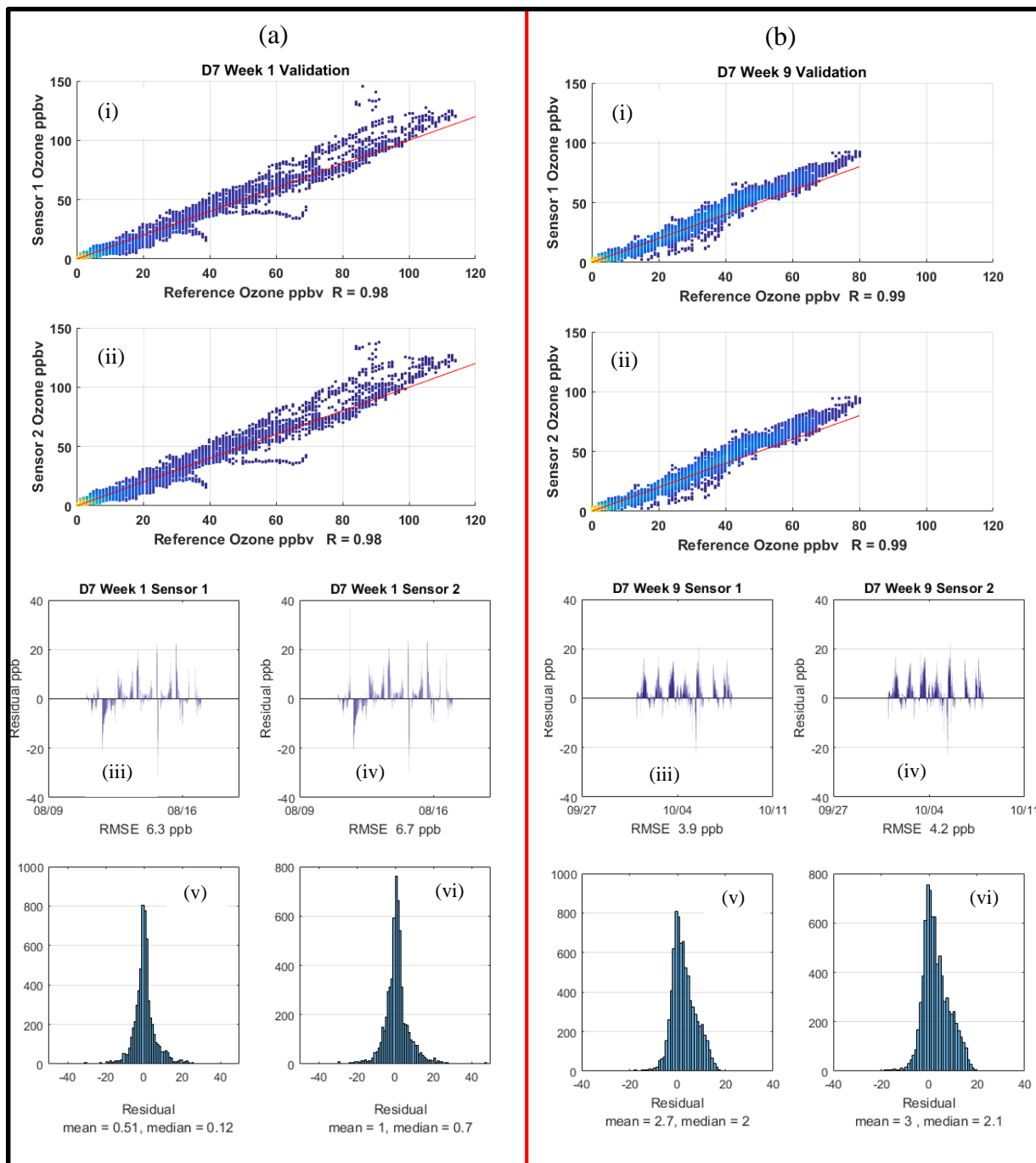
Figure 6: Validation results from the (a) first week and (b) ninth week of the deployment period for D7 ozone sensors separated by the red line. Subpanels (i) show a scatterplot of sensor 1 and reference measurements with warmer shading showing a higher density of points, (ii) show a scatterplot of sensor 2 and reference measurements with warmer shading showing a higher density of points, (iii) depict residuals over time for sensor 1 with RMSE, (iv) depict residuals over time for sensor 2 with RMSE, (v) is a histogram of residuals with mean and median residual for sensor 1, (vi) is a histogram of residuals with mean and median residual for sensor 2.
