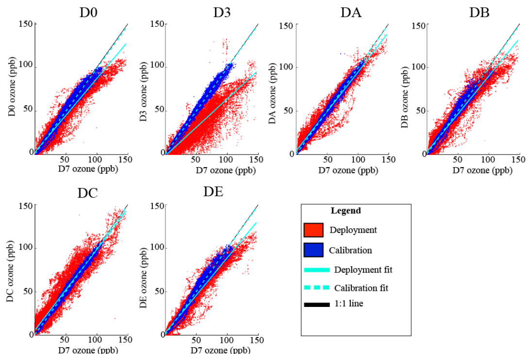
15 Figure 10. U-Pod D7 ozone concentrations are plotted on the x-axis and other U-Pod ozone concentrations recorded at the same times are on the y-axis. The sets are color coded according to time period their data were taken, and each color is fit with a linear line.
