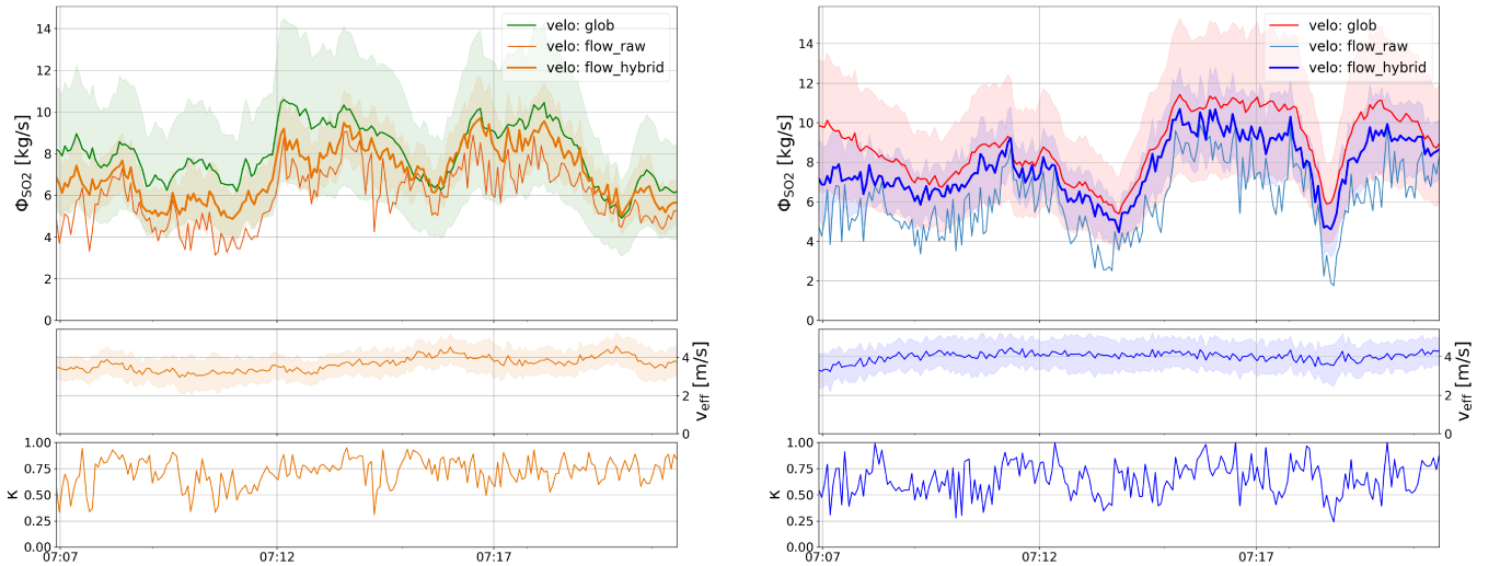
Figure 6. Time series of Etna emission-rates (top panel), showing emissions of the young (left) and the aged (right) plume of the NE crater (orange/blue colours, respectively) using the two PCS lines shown in Fig. 1. Emission rates were retrieved using the three different velocity retrieval methods described above. Uncertainties (shaded areas) are only plotted for the flow_hybrid method and the cross-correlation method (“glob”). Further included are time series of effective velocities (Eq. 4, middle panel) and \kappa values (Eq. 7, bottom) retrieved from the proposed histogram analysis.
