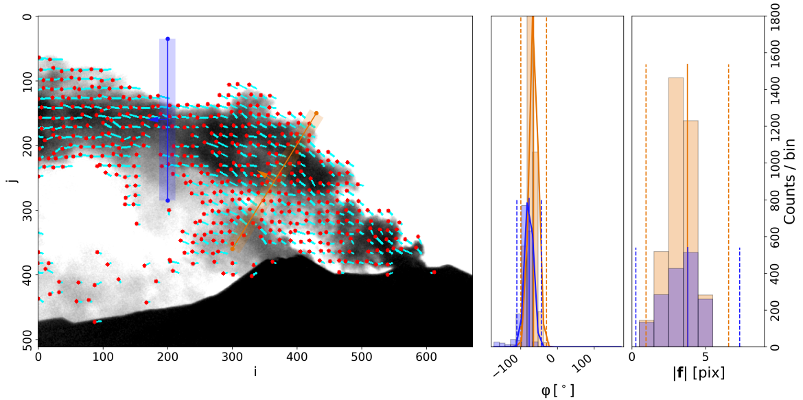
Figure 4. Left: Example flow vector field (blue lines with red dots) of the Farnebäck optical flow algorithm for the Etna plume at 07:13 UTC including the two PCS lines (blue / orange) and the corresponding ROIs used for the histogram analysis (semi-transparent rectangles). Middle, right: histograms of orientation angles \mathcal{M}_\phi and vector magnitudes \mathcal{M}_{|f|} for both lines (bar plot), determined using condition S7 in Appendix A1. The \mathcal{M}_\phi histogram (middle) also includes fit results of the Multi-Gauss peak detection (thick solid lines). The retrieved histogram parameters ( \phi_\mu , |f|_\mu ) and expectation intervals \mathcal{M}_\phi , \mathcal{M}_{|f|} are indicated with solid and dashed vertical lines, respectively. From the corrected DVF , average effective velocities of v_{\text{eff}} = (3.9 \pm 0.5) \text{ m/s} (orange line) and v_{\text{eff}} = (4.4 \pm 0.8) \text{ m/s} (blue line) were retrieved. Note that in the left image 1) vectors shorter than 1.5 pixels are excluded, 2) the displayed vector lengths were extended by a factor of 3 and 3) only every 15th pixel of the DVF is displayed.
