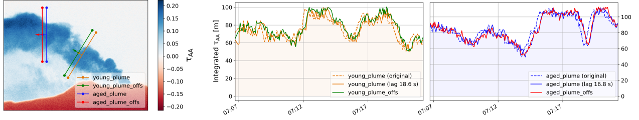
Figure 14. Result of velocity cross-correlation analysis for the Etna data. Left: Example plume AA image including two PCS lines (orange / blue) and corresponding offset lines (green / red) used for the analysis. Middle, right: corresponding time series of the integrated AA values along the two PCS lines (original: dashed, shifted using correlation lag: solid) and along the offset lines (solid) using the same colour scheme.
