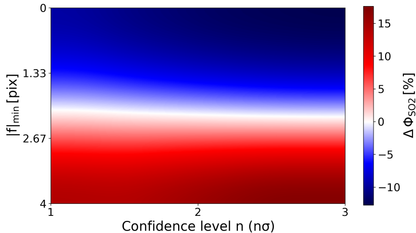
Figure 16. Sensitivity of SO 2 emission-rates as a function of the chosen input settings |f|_{\min} (y-axis) and the confidence level n (x-axis). The investigated value ranges are 0–4 pixels for |f|_{\min} and 1–3 for the n and the deviations are plotted as percentage deviations \Delta\Phi_{\text{SO}_2} from the average SO 2 emission-rate retrieved from this study. The latter amounts to 2.4 kg/s (not dilution corrected, see text). The analysis was performed using the average SO 2 emission-rates retrieved from 30 images of the Etna dataset.
