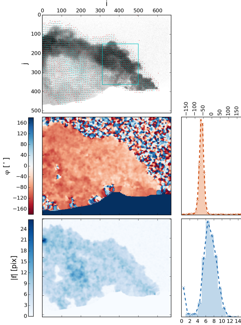
Figure 3. Example output of the Farnebäck optical flow algorithm including a rectangular ROI (top). Two further images show the corresponding orientation angles \varphi (middle) and magnitudes |\mathbf{f}| (bottom) of the DVF . Corresponding histograms \mathcal{M}_\varphi and \mathcal{M}_{|\mathbf{f}|} are plotted on the right, respectively, and include all pixels in the displayed ROI. The histograms are plotted both including (dashed lines) and excluding (red / blue shaded areas) short flow vectors (i.e. |\mathbf{f}| > |\mathbf{f}|_{\min} = 1.5\text{pix} ). The orientation angles are plotted in an interval -180^\circ \leq \varphi \leq +180^\circ where -90^\circ , +90^\circ correspond to -i , +i directions, respectively and 0^\circ to the vertical upwards direction ( -j ). The DVF was calculated using two consecutive AA images ( \Delta t = 4.0\text{s} ) of the Etna plume, recorded on 16/09/2015 at 07:14 a.m.
