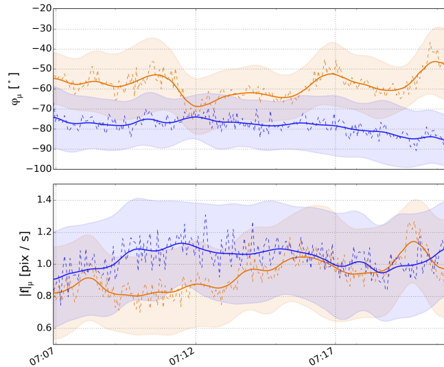
Figure 5. Time series of retrieved PDV parameters \varphi_\mu and |f|_\mu (dashed lines) for the two Etna PCS lines (same colours, cf. Fig. 1) and corresponding values after applying interpolation and smoothing (solid lines). The expectation intervals \mathcal{I}_\varphi and \mathcal{I}_{|f|} are plotted as shaded areas.
