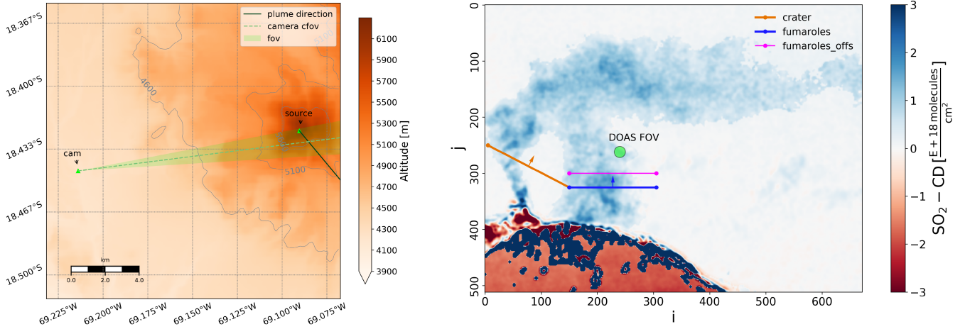
Figure 2. Left: Guallatiri overview map showing position and viewing direction of camera ( camera cfov , fov ), summit area ( source ) as well as the plume azimuth ( plume direction ). Right: example SO 2 -CD image of the Guallatiri emissions including two PCS lines used to retrieve SO 2 emission-rates from the central crater (orange) and from a fumarolic field (blue) located behind the flank in the viewing direction. An additional line (magenta) is used to estimate gas velocities using a cross-correlation algorithm (relative to blue PCS line, cf. Appendix B4). Position and extent of the DOAS-FOV is indicated by a green spot. Note that the displayed plume image is size reduced by a factor of two (Gauss pyramid level 1).
