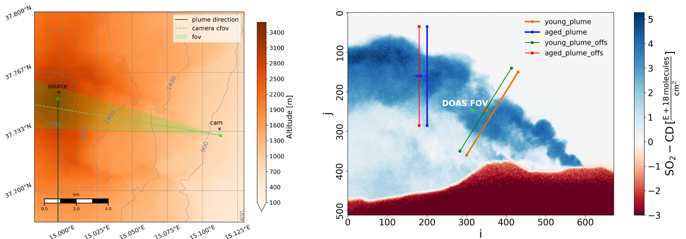
Figure 1. Left: Etna overview map showing position and viewing direction of the camera ( camera cfov , fov ) which was located on a roof-top in the town of Milo. Also indicated is the summit area ( source ) and the plume azimuth ( plume direction ). Right: example SO 2 -CD image of the Etna plume including two PCS lines (orange / blue) used for emission-rate retrievals and two corresponding offset lines (green, red), that are used for cross-correlation based plume velocity retrievals (cf. Appendix B4). Position and extent of the DOAS-FOV for the camera calibration is indicated by a green spot. Note that the displayed plume image is size reduced by a factor of two (Gauss pyramid level 1).
