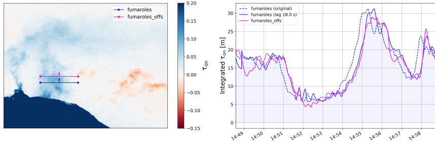
Figure 15. Result of velocity cross-correlation analysis for Guallatiri data. Left: Example plume on-band OD image ( \tau_{on} ) including the PCS (blue) and offset line (magenta) used for the analysis. Right: corresponding time series of integrated on-band ODs (dashed blue / magenta) and further, the shifted PCS signal corresponding to the retrieved correlation lag of 18.0 s (solid blue). Note that here, the velocity analysis was applied using a time series of on-band OD images rather than the \tau_{AA} which was used in Fig. 14.
