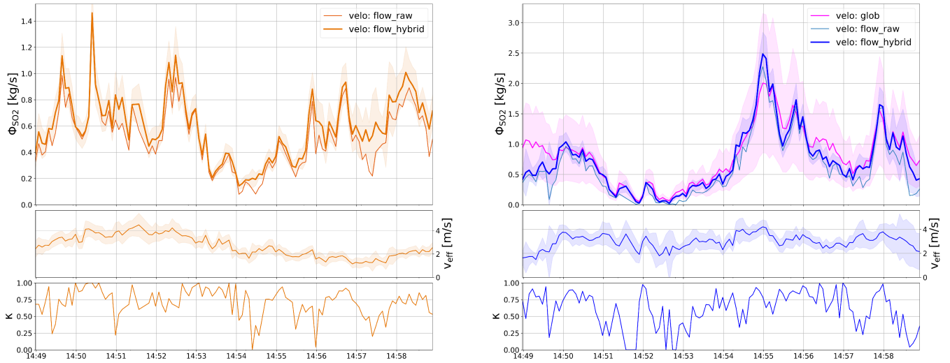
Figure 10. Guallatiri \text{SO}_2 emission-rates from the summit crater (left, orange colours) and the fumarolic field (right, blue colours) using the two PCS lines shown in Fig. 2. Uncertainties (shaded areas) are only plotted for the flow_hybrid and the glob (cross-correlation based velocity) retrieval methods. Further included are the corresponding effective velocities (from the flow_hybrid method) and the OF quality factors \kappa (Eq. 7). The central crater emissions show only little variability ( \Phi \approx 0.6 \text{ kg/s} ) while the fumarolic emissions are characterised by a comparatively strong emission “event” at 14:55 UTC showing peak emissions of 2.5 \text{ kg/s} .
