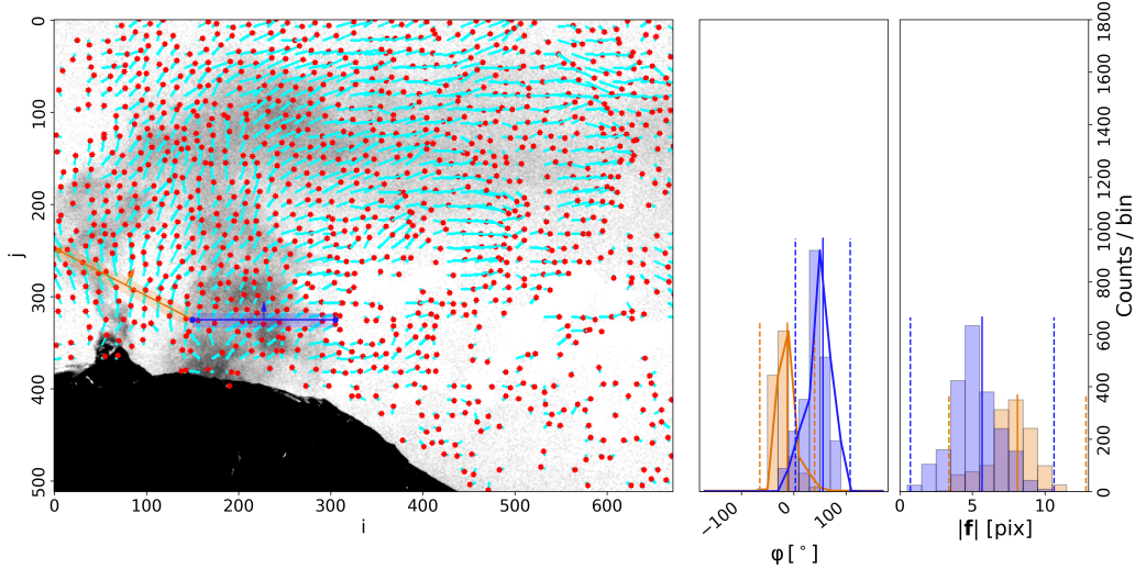
Figure 8. Left: Example output of the Farneback optical flow algorithm for the Guallatiri emissions at 14:48 UTC including the two example PCS lines (blue / orange line) and the corresponding ROIs. Middle and right: Histograms of magnitudes \mathcal{M}_\varphi and orientation angles \mathcal{M}_{|f|} used to retrieve the expectation intervals \mathcal{I}_\varphi and \mathcal{I}_{|f|} and the corresponding PDV in each ROI, respectively (cf. Eq. 5). From the latter, effective velocities of \mathbf{v}_{\text{eff}} = (3.1 \pm 0.5) \text{ m/s} (crater, orange) and \mathbf{v}_{\text{eff}} = (1.8 \pm 0.6) \text{ m/s} (fumaroles, blue) were retrieved. Note that in the left image 1) vectors shorter than 1.5 pixels are excluded, 2) the displayed vector lengths were extended by a factor of 2 and 3) only every 15th pixel of the DVF is displayed.
