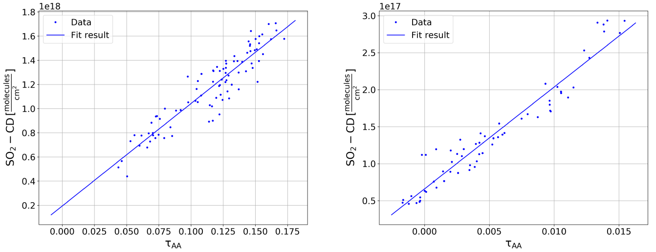
Figure 13. DOAS calibration curves of Etna data (left) and Guallatiri data (right) retrieved from AA images (not dilution corrected) within the image region covered by the DOAS-FOV (cf. Figs. 1 and 2). The corresponding \text{SO}_2 -CDs retrieved with the DOAS instrument are plotted on the y-axis. Y-axis offsets were corrected for during the calibration of the AA images.
