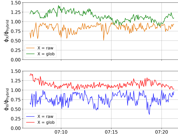
Figure 7. Relative deviations of retrieved SO 2 emission-rates shown in Fig. 6 for the “young_plume” (top) and the “aged_plume” (bottom) PCS lines using the same colour codes as in Fig. 6. The ratios are plotted relative to the results of the proposed flow_hybrid method. Results based on the cross-correlation analysis tend to be slightly larger (by about +14%) while the uncorrected OF velocities often yield underestimated SO 2 emission-rates (up to 62%).
