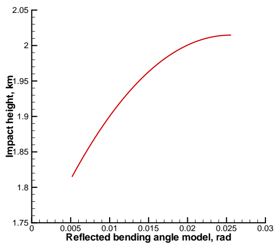
Figure 6. Reflected bending angle model for occultation event 2008/01/01, UTC 01:02:23, 70.28°N 121.87°W (the same event as in Figure 2).
