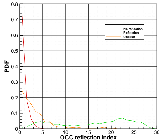
Figure 14. Probability distribution function of I_R for the three categories of events.
