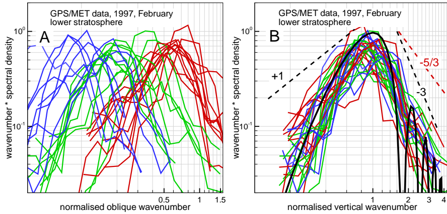
Figure 2. Amplitude fluctuation spectra for the lower stratosphere: panel A: spectra as functions of the oblique wavenumber corresponding to the isotropy hypothesis (Kolmogorov turbulence); panel B: spectra as functions of the vertical wavenumber corresponding to the anisotropy hypothesis (saturated IGWs). The color map red–green–blue corresponds to the increasing obliquity angles, which are subdivided into three groups. The black solid line in panel B presents the theoretical vertical spectrum for the saturated IGW model; the dashed lines present the asymptotics of this spectrum for low and high frequencies, the low-frequency asymptotic is evaluated for L_W \rightarrow \infty . For the comparison, red dashed lines show the high-frequency spectral asymptotic of the Kolmogorov turbulence model.
