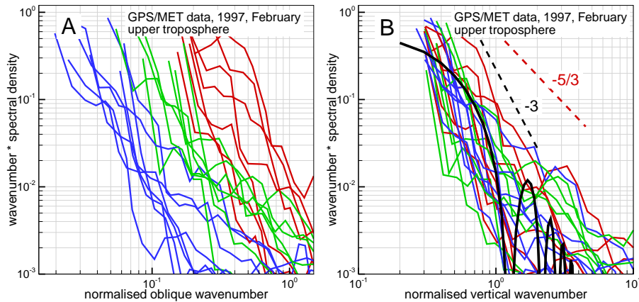
Figure 5. The normalized eikonal fluctuation spectra for the upper troposphere. Panel A: spectra as functions of the oblique wavenumber corresponding to the isotropy hypothesis; panel B: spectra as functions of the vertical wavenumber corresponding to the anisotropy hypothesis. The notations are the same as in Figure 4.
