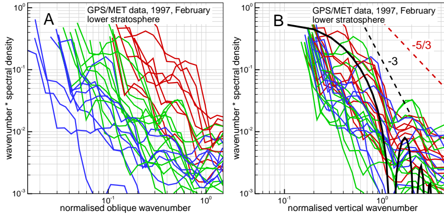
Figure 4. The normalized eikonal fluctuation spectra for the lower stratosphere: panel A: spectra as functions of the oblique wavenumber corresponding to the isotropy hypothesis; panel B: spectra as functions of the vertical wavenumber corresponding to the anisotropy hypothesis. The black solid line in panel B represents the theoretical vertical spectrum for the saturated IGW model; the dashed line represents its asymptotics. For the comparison, red dashed lines show the high-frequency spectral asymptotic of the Kolmogorov turbulence model. Cf. the caption of Figure 2.
