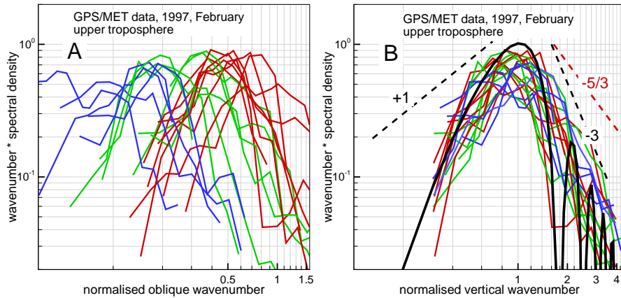
Figure 3. Amplitude fluctuation spectra for the upper troposphere: panel A: spectra as functions of the oblique wavenumber corresponding to the isotropy hypothesis (Kolmogorov turbulence); panel B: spectra as functions of the vertical wavenumber corresponding to the anisotropy hypothesis (saturated IGWs). The notations are the same as in Figure 2
