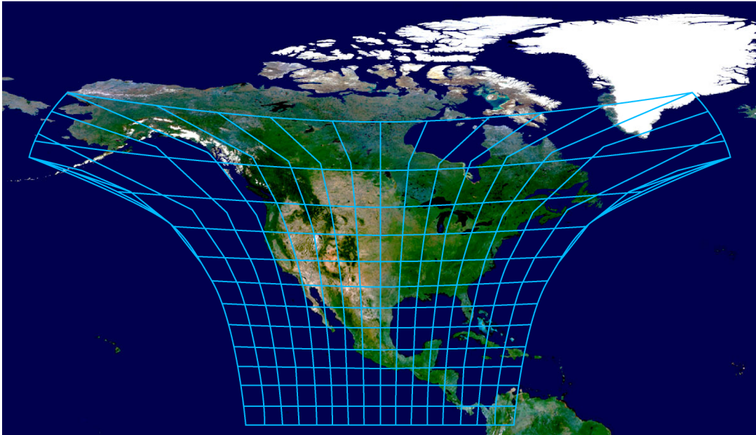
505 Figure 8: CHRONOS field of view from geostationary orbit at 100° W. Each grid cell above represents 125 x 125 pixels. All pixels are acquired with full precision within the ~10 minute CHRONOS data acquisition.
