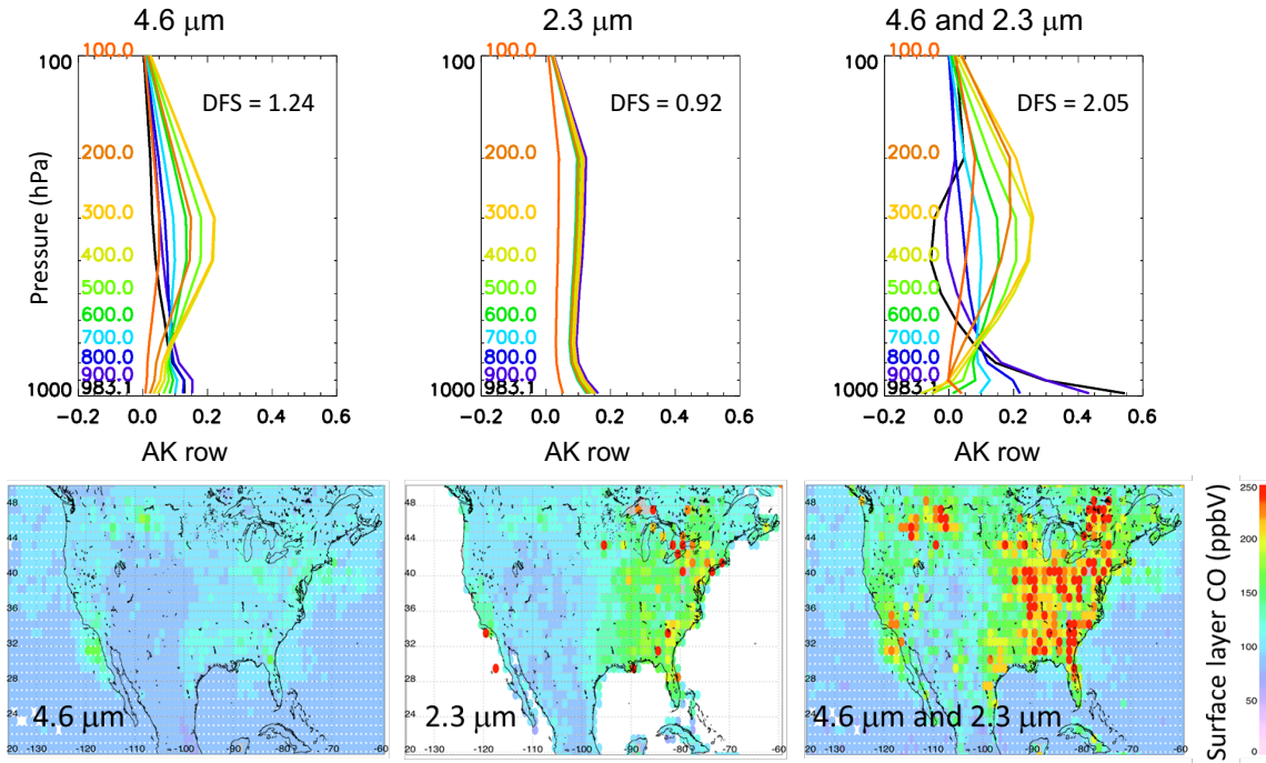
Figure 13: Comparison of surface layer CO for MOPITT version 7 data (Deeter et al., 2017)
