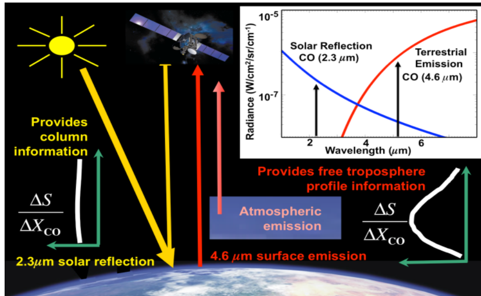
Figure 12: Physics of CHRONOS and MOPITT multispectral measurements. In the SWIR at 2.2 and 2.3 μm, measurement signals rely on daytime reflected solar radiation and weak spectral features. Changes in CH 4 and CO mixing ratios, ΔX, produce uniform signal sensitivity, ΔS, throughout the vertical profile, including near the surface. In the MWIR at 4.6 μm, signal sensitivity is greatest in the middle troposphere, except in cases of high thermal contrast between the surface and the lowest atmospheric layers. CHRONOS CH 4 SWIR retrievals use the solar reflected radiance to provide a true total column, and CO multispectral retrievals combine the SWIR and MWIR measurements to increase the sensitivity to near-surface CO. While this increased sensitivity varies depending on scene characteristics such as albedo, in many cases, it provides improved information to distinguish local air pollution emissions and transported plumes.
