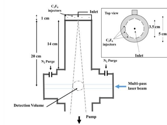
Figure 2. Schematic of the IU-FAGE sampling/excitation axis (left) and cross section with dimensions for the medium inlet configuration (right).
