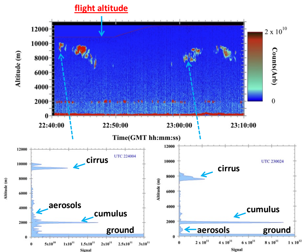
Figure 1. A 30-minute long vertical cross-section (top panel) and two individual 1-s vertical profiles (bottom panels) of atmospheric backscattering at off-line wavelengths of \text{CO}_2 line measured by NASA GSFC \text{CO}_2 Sounder near West Branch Iowa tall tower site on Aug. 11, 2011. The backscatter signals were corrected by square of range and averaged by 1 \mu\text{s} vertical running mean (150-m) and 1-s horizontal running mean (200-m of ground track). Returns from ground, cumulus and cirrus clouds, and aerosols are illustrated and labeled.
