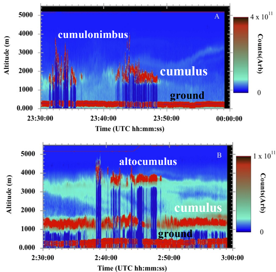
Figure 11. Vertical cross-sections of range-corrected backscattered pulse energy for Segment A and B marked in Fig. 10. The lidar returns from the ground are at the bottom and cloud returns are at a variety of altitudes from 1 to 4 km. The red lines on the top of plots indicate aircraft flight altitudes.
