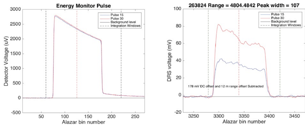
Figure 7. The lidar transmitted pulse shape (left panel) and the recorded echo pulse shape returned from a cloud top (right panel). The blue lines are for pulse #15 that is near CO 2 absorption line center and the red lines are for pulse #30 in the line wing.
