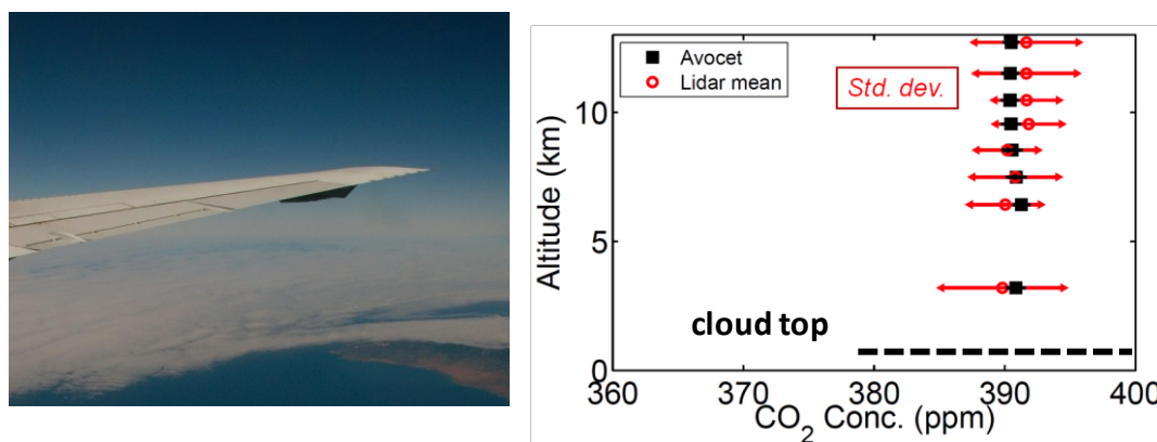
Fig. 8. (Left panel) Photo of marine stratus cloud deck over the Pacific Ocean near the California coastline taken on the ASCENDS flight on Aug. 2, 2011. (Right panel) The retrieved values of XCO 2 to the cloud tops at altitudes of 700-m (black dashed line) as a function of flight altitude. The XCO 2 values integrated from in situ AVOCET gas analyzer are marked in black squares and the retrieved values from the CO 2 Sounder for 10-s average are marked in red circles. The error bars for the retrieved XCO 2 are for ±1 standard deviation.
