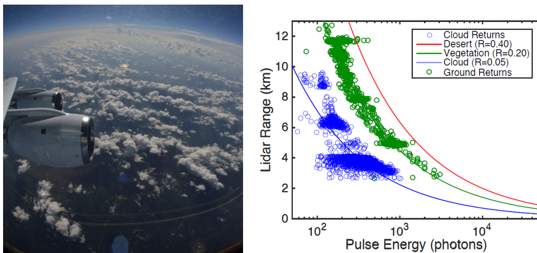
5 Figure 6. The left photo shows the cumulus clouds above PBL from the ASCENDS sunset flight on Aug. 25, 2014 near the West Branch Iowa tall tower. The right panel shows the returned pulse energy in number of photons as a function of lidar range from airplane altitude for the cumulus clouds. The average ground reflectance (in green) is approximately 20%, while the average cumulus cloud top reflectance is about 5% (in blue) and shows more variability.
