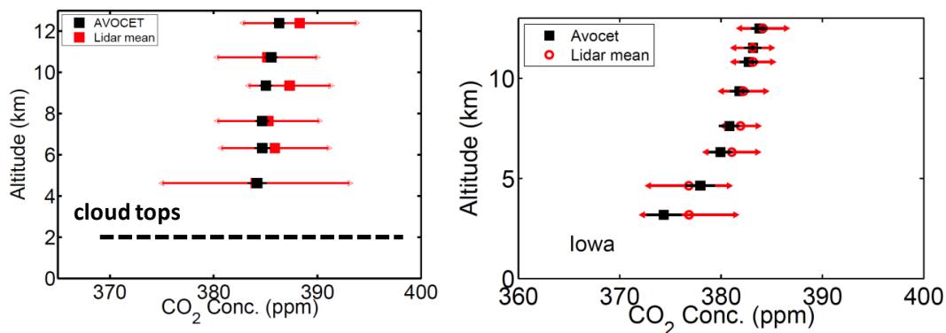
Figure 9. The XCO 2 retrievals for lidar measurements to the tops of broken cumulus clouds (left panel) and to the ground (right panel) on the Aug. 10, 2011 ASCENDS flight over Iowa. The XCO 2 values from in situ AVOCET gas analyzer are marked in black squares and the values of XCO 2 retrievals from CO 2 Sounder measurements averaged over 10 seconds are marked in red circles with error bars of \pm 1 standard deviation. The average altitude of cloud tops (~2 km) is plotted in the dashed line.
