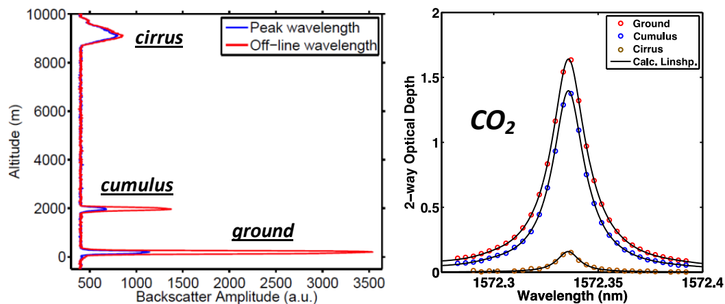
5 Figure 2. Backscatter profile (left panel) and CO 2 absorption line shapes (right panel) in terms of optical depth for laser returns from ground, cumulus clouds and cirrus clouds near West Branch Iowa tall tower site on Aug. 10, 2011. In the left panel, the backscatter profile of off-line is plotted in red, and the backscatter profile at line center with peak absorption is plotted in blue. Both optical depth and differential optical depth between off-line and line center wavelength increases with photon path length or range between airplane and the scattering surface. Data are averaged over 10-s of ground track for both plots. In the right panel the dots are the lidar measurements and the solid lines are the best-fit line shapes from the XCO 2 retrievals.
