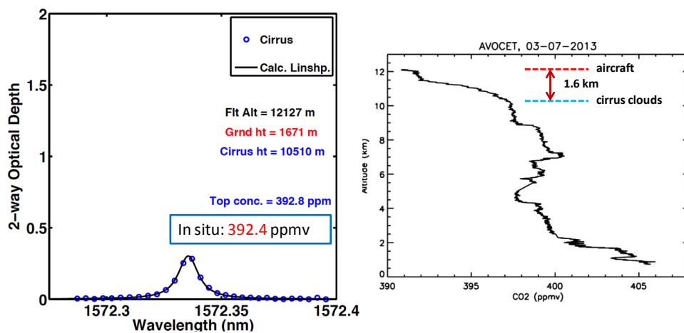
5 Figure 13. A CO 2 absorption line shape measured on the March 7, 2013 to cirrus cloud tops at 10.5 km altitude (left panel). The lidar measurements are the blue circles and the fitted line shape is the solid black line. AVOCET in situ vertical profile of CO 2 concentration is plotted at the right panel. The aircraft flight altitude was 12.1 km and the lidar range to cirrus cloud tops was 1.6 km.
