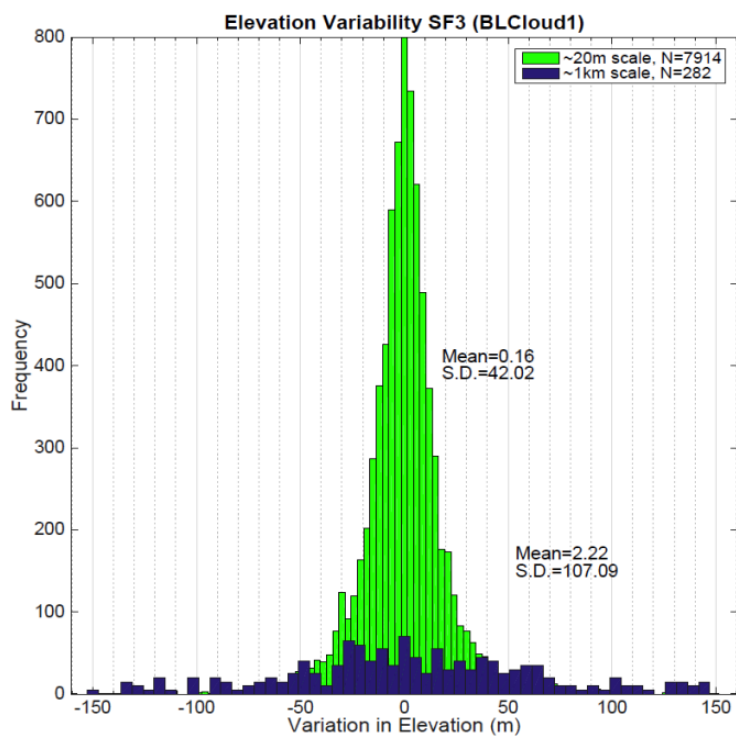
Figure 5. Same as Fig. 4 for the Aug. 25, 2014 flight above cumulus clouds in Iowa, showing a 0.1-s standard deviation of 42 m and a 5-s standard deviation of 107 m.
