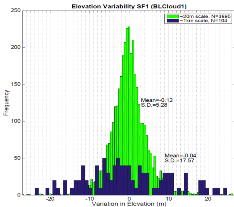
Figure 4. Histogram of the variation in cloud top height after averaged for 0.1-s (in green) and 5-s (in blue), respectively, for the Aug. 20, 2014 flight above stratus clouds along California coastline, showing a 0.1-s standard deviation of 5.2 m and a 5-s standard deviation of 18 m..
