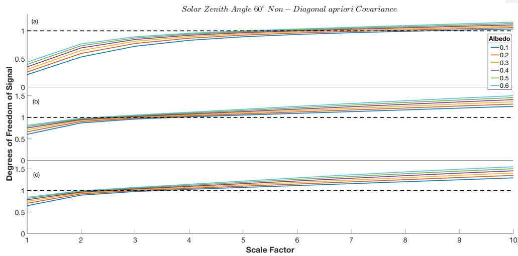
Figure A2. Degrees of Freedom for ^{13}\text{CH}_4 vs scaling factor f for scenarios outlined in Table 3. Each coloured line represents different surface albedo conditions as shown in the key. The black dashed line represents unity DOFS: (a) indicates scenario 3, (b) indicates scenario 6, (c) indicates scenario 9.
