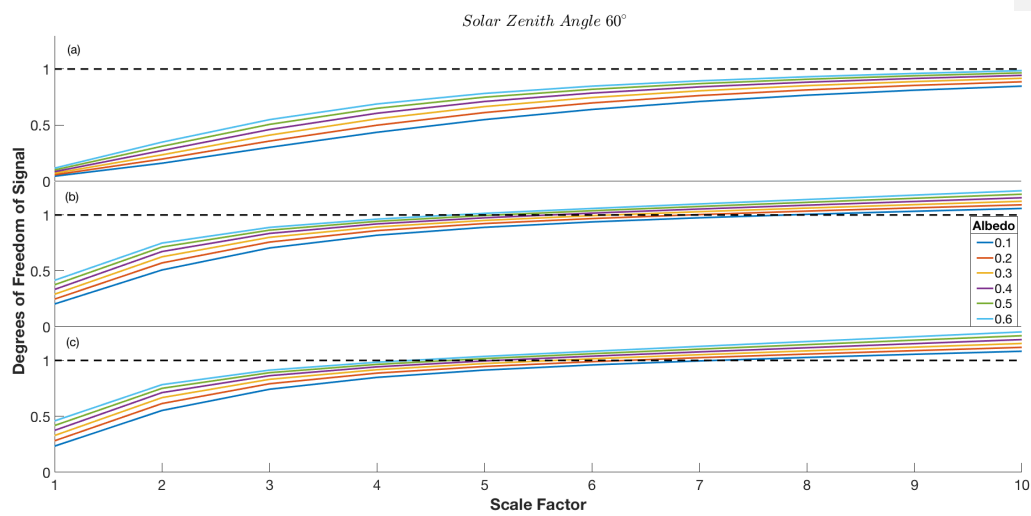
Figure A1. Degrees of Freedom for ^{13}\text{CH}_4 vs scaling factor f for scenarios outlined in Table 3. Each coloured line represents different surface albedo conditions as shown in the key. The black dashed line represents unity DOFS: (a) indicates scenario 2, (b) indicates scenario 5, (c) indicates scenario 8.
