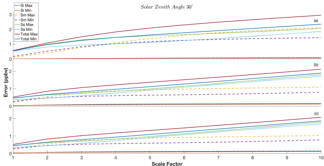
Figure 7. Synthetic total column retrieval errors for scenarios outlined in Table 3, based on Eqs. (8,9,10 & 16). The maximum and minimum values (based on maximum and minimum SNR), for interference, measurement and smoothing error are shown, in addition to the total error: a) indicates scenario 1, b) indicates scenario 4, c) indicates scenario 7.
