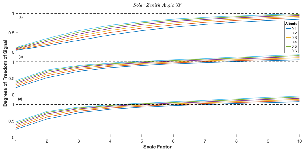
Figure 6. Degrees of Freedom for Signals for ^{13}\text{CH}_4 vs scaling factor f for scenarios outlined in Table 3. Each coloured line represents different surface albedo conditions as shown in the key. The black dashed line represents unity DOFS: a) indicates scenario 1, b) indicates scenario 4, c) indicates scenario 7.
