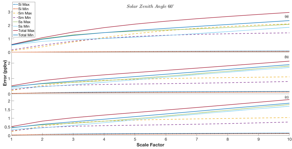
Figure A3. Synthetic total column retrieval errors retrieval for scenarios outlined in Table 3, based on Eqs. (8,9,10 & 16). The maximum and minimum values (based on maximum and minimum SNR), for interference, measurement and smoothing error are shown, in addition to the total error: a) indicates scenario 2, b) indicates scenario 5, c) indicates scenario 8.
