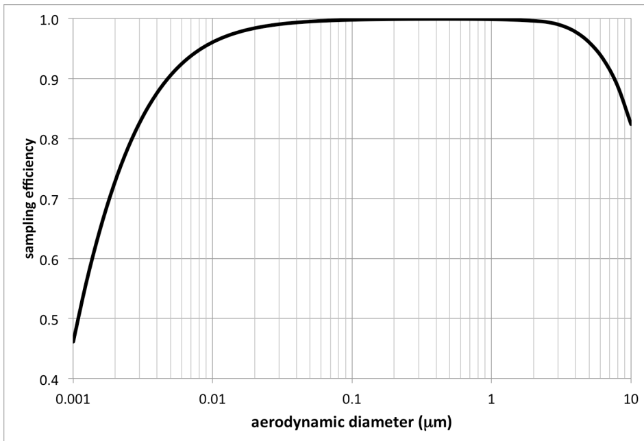
Figure 2: Calculated sample efficiency of particles reaching the CLAP filter
