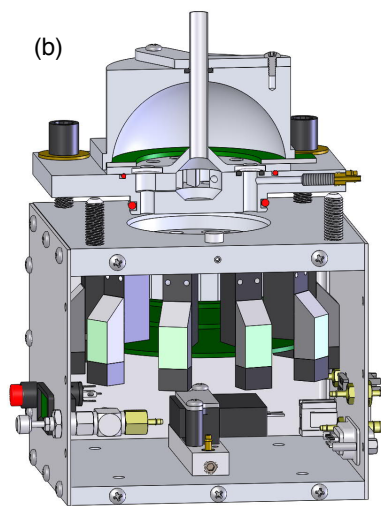
Figure 1: (a) Photograph of CLAP, and (b) cross-sectional view of flow and optical paths in upper section and three-dimensional view of CLAP internal configuration in lower section. Scale on ruler in left image is in millimeters. An annotated version of (b) is included in the Supplement (Fig. S1).
