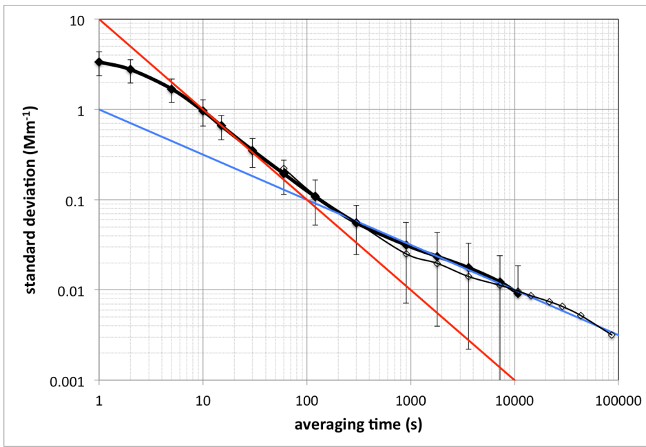
Figure 6: Standard deviation of attenuation coefficient measured on filtered air, as a function of averaging time. Thick black line with solid symbols represents the measurement data based on 8 h of measurements/spot; thin black line with open symbols shows the measurement data when each spot was sampled for 1 week; red line represents approximate slope for 5-100 s averaging time; blue line represents approximate slope for 2 min to 1 day averaging times.
