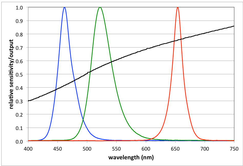
Figure 3: Normalized spectral output of light source for blue, green, and red channels, and spectral sensitivity of detector (black curve).
