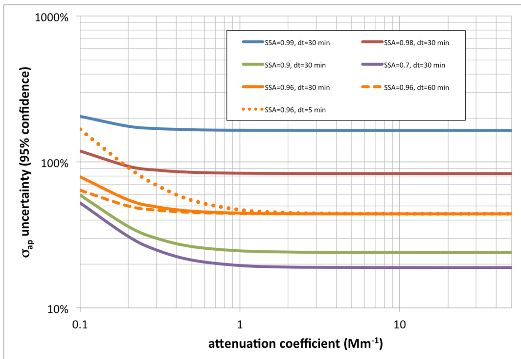
Figure 8: Uncertainty of CLAP measurements of absorption coefficient (95% confidence level) as a function of attenuation coefficient, for various values of single-scattering albedo (SSA) and averaging time (dt). Solid lines are all for 30 min averaging time, dashed lines are for other averaging times as noted in the legend
