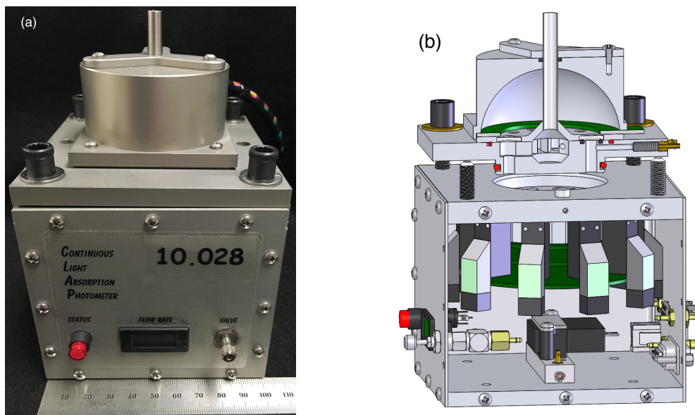
5 Figure 1: (a) Photograph of CLAP, and (b) cross-sectional view of flow and optical paths in upper section and three-dimensional view of CLAP internal configuration in lower section. Scale on ruler in left image is in millimeters. An annotated version of (b) is included in the Supplement (Fig. S1).
