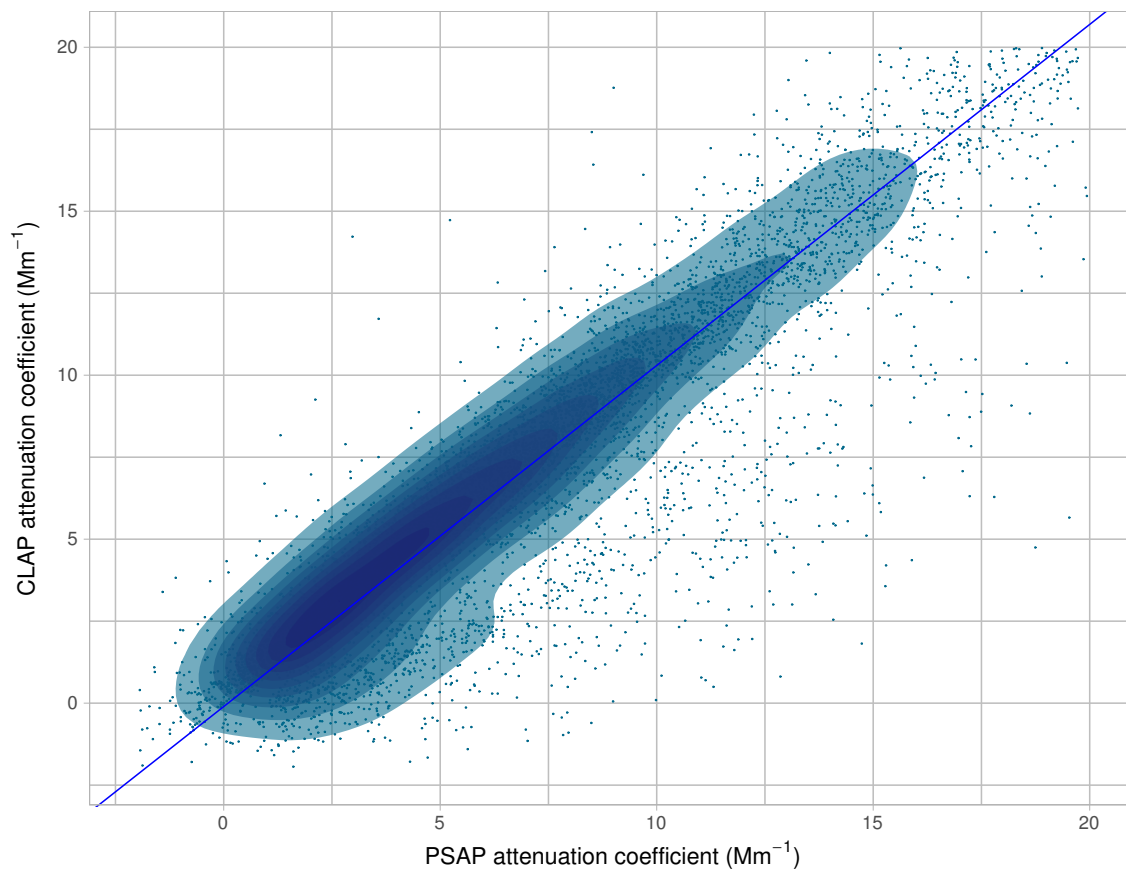
5 Figure 10: Comparison of attenuation coefficients measured with CLAP and PSAP. Results represent 8442 30-minute averages for Bondville, IL, USA (PM10 size range, blue wavelength channel). The shaded areas contain 90% of the observations and the color shading distinguishes the deciles of the two-dimensional probability distribution function. The slope of the regression line is 1.04 with an intercept of -0.10; the regression line accounts for 98% of the variance in the measured data.
