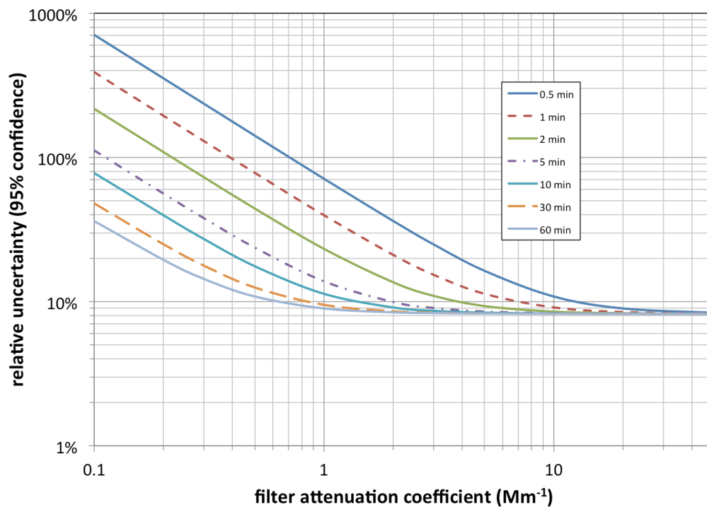
Figure 7: Uncertainty of CLAP measurements of attenuation coefficient as a function of averaging time and attenuation coefficient, expressed as the 95% confidence level.
