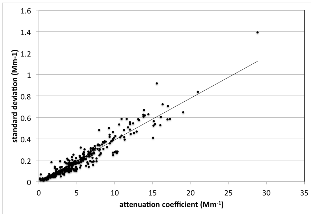
Figure 5: Standard deviation of attenuation coefficient measured by nine CLAPs (1-hr averages, 529 nm wavelength). Line indicates slope of regression, forced through the origin.
