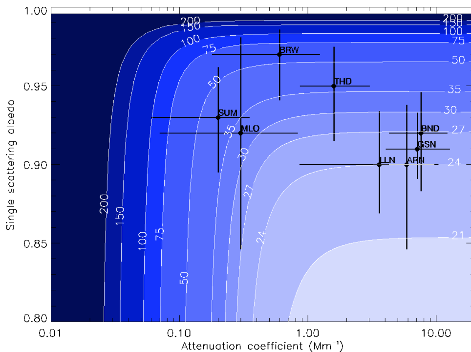
Figure 9: Percent uncertainty of 30-min average light absorption coefficient as a function of single-scattering albedo and attenuation coefficient. The median uncertainty and inter-quartile range are shown for values measured for 2013-2016 at eight sites (ARN, El Arenosillo, Spain; BND, Bondville, USA; BRW, Barrow, USA; GSN, Gosan, South Korea; LLN, Mt. Lulin, Taiwan; MLO, Mauna Loa, Hawaii; SUM, Summit, Greenland; THD, Trinidad Head, USA). Uncertainties are given at the 95-percent confidence level.
