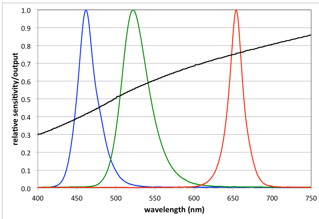
Figure 3: Normalized spectral output of light source for blue, green, and red channels, and spectral sensitivity of detector (black curve).
