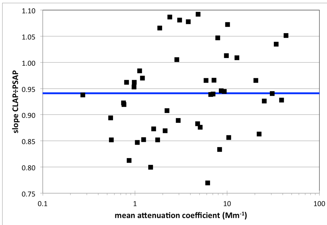
Figure 11: Slope of orthogonal regression line relating attenuation coefficients measured by CLAP vs. PSAP as a function of mean attenuation coefficient for 17 stations. The blue line indicates the mean slope of 0.941. Data are given for all measured wavelengths.
