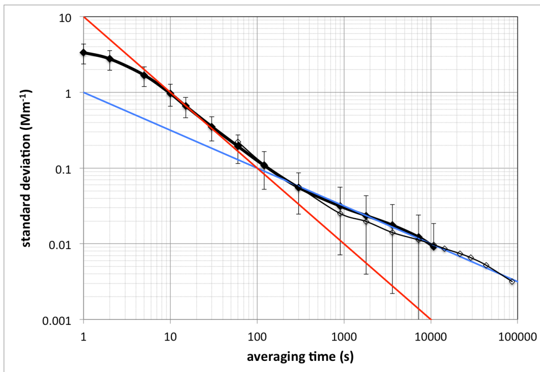
5 Figure 6: Standard deviation of attenuation coefficient measured on filtered air, as a function of averaging time. Thick black line with solid symbols represents the measurement data based on 8 h of measurements/spot; thin black line with open symbols shows the measurement data when each spot was sampled for 1 week; red line represents approximate slope for 5-100 s averaging time; blue line represents approximate slope for 2 min to 1 day averaging times.
