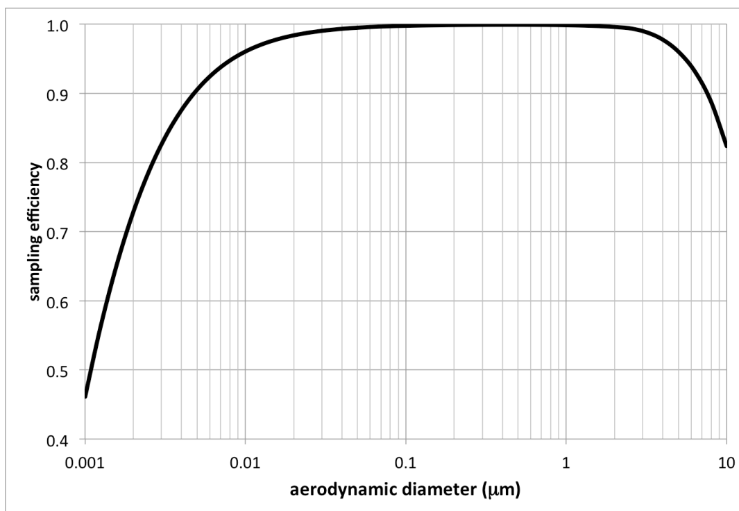
Figure 2: Calculated sample efficiency of particles reaching the CLAP filter
