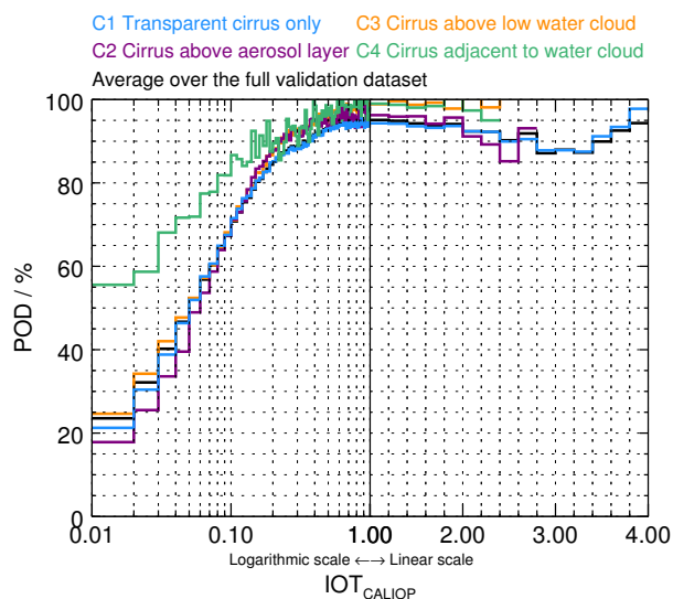
Figure 6. The cirrus POD of CiPS as a function of the IOT retrieved by CALIOP for the vertical cloud-aerosol structure classes C1-C4 along with the average POD over the full validation dataset.
