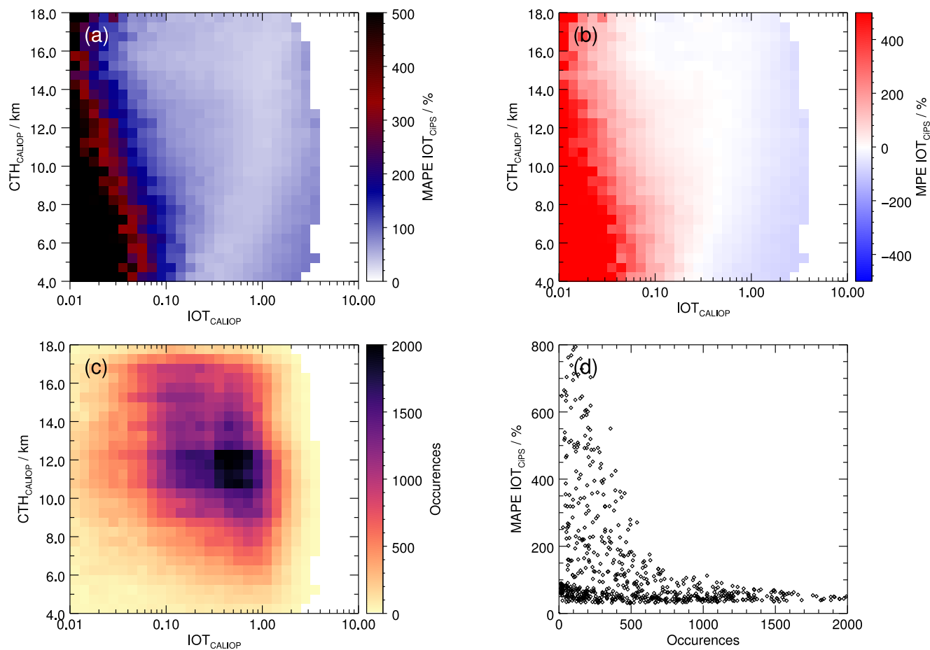
Figure 10. (a) 2D histogram showing the MAPE of the IOT_{CIPS} retrievals as a function of the reference IOT_{CALIOP} and CTH_{CALIOP} . (b) 2D histogram showing the MPE of the IOT_{CIPS} retrievals as a function of IOT_{CALIOP} and CTH_{CALIOP} . (c) 2D histogram showing the number of occurrences for different combinations of IOT_{CALIOP} and CTH_{CALIOP} . (d) The MAPE of the IOT_{CIPS} retrievals for the different IOT_{CALIOP}/CTH_{CALIOP} combinations as a function of the number of occurrences (each diamond represents two corresponding grid boxes in (a) and (c)).
