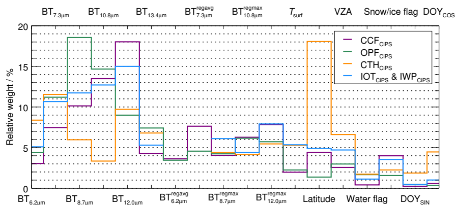
Figure 1. Relative weight of the CiPS input variables for the 4 ANNs. BT = Brightness Temperature, regavg = regional average, regmax = regional maximum, VZA = viewing zenith angle, DOY_{SIN} = \sin(2\pi DOY/365) and DOY_{COS} = \cos(2\pi DOY/365) .
