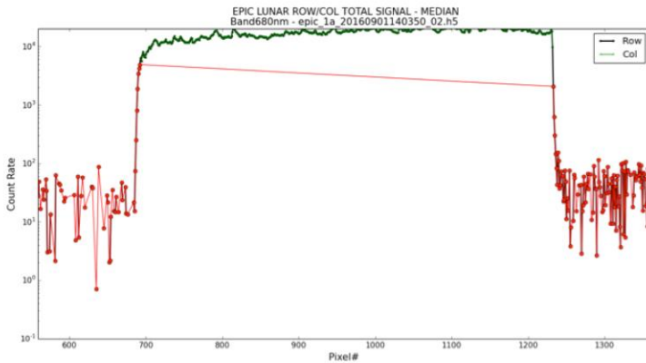
Examples of moon observations in 680 (left) and 688 (right) on 09/01/2016 (courtesy of Matthew Kowalewski).
