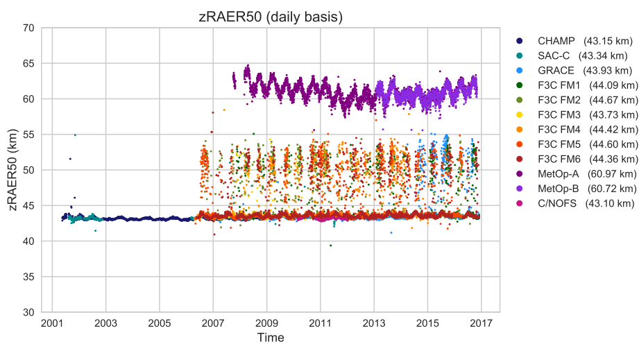
Figure 7. Temporal evolution of daily median zRAER50 for all RO missions processed in OPSv5.6. The mean of zRAER50 is shown as value in parantheses in the legend. Only high-quality profiles are used in these statistics.
