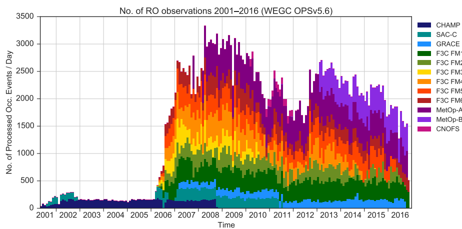
Figure 5. Daily number of high-quality OPSv5.6 profiles for different satellites (different colors) as a function of time from 2001 to 2016.
