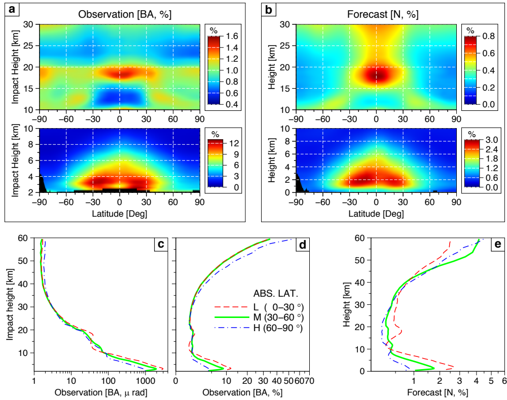
Figure 1. An example of diagonal elements of a) \mathbf{R} and b) \mathbf{B} diagnosed with HL86. Shown are the error standard deviations (%) of a) observed bending angle and b) forecast refractivity, averaged along the longitude and over the whole data period. The bending angle \sigma_o averaged in three latitude bands (low latitude, red dashed; middle latitude, solid green; high latitude, blue dashed dot) is shown in the unit of c) 10^{-6} rad and d) %. e) is the same as in d) except for refractivity \sigma_f .
