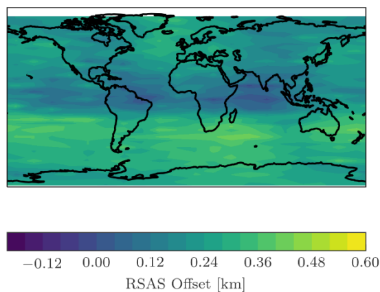
5 Figure 3: Globally binned in latitude and longitude RSAS offsets for time period beginning in 2004 and ending in 2010. Values where the OSIRIS optics temperature is less than 18° C are excluded.
