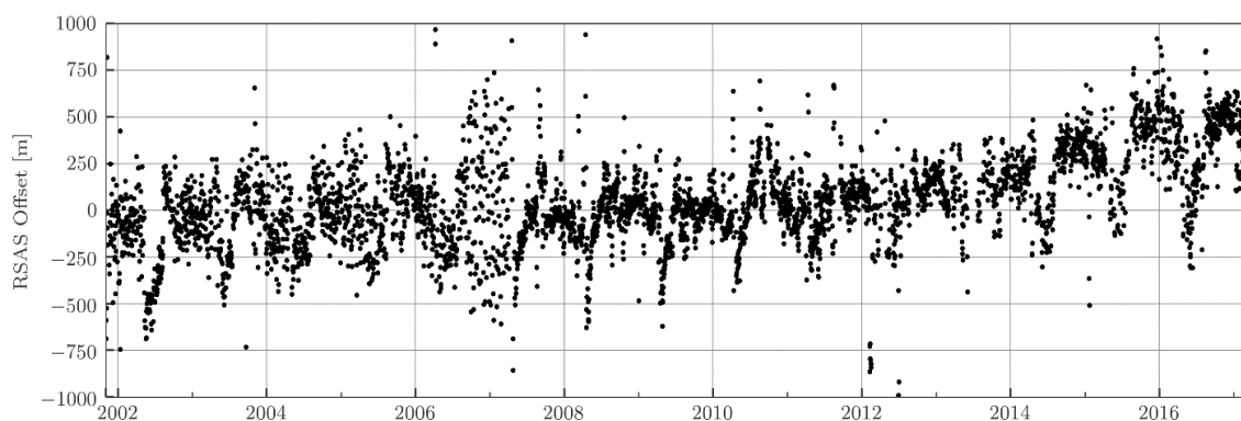
Figure 4: Daily average RSAS tangent height offset after subtracting the geographic average from GEOGRAPHIC AVERAGE FIGURE. This is the final correction that is used in v5.10 data processing.
