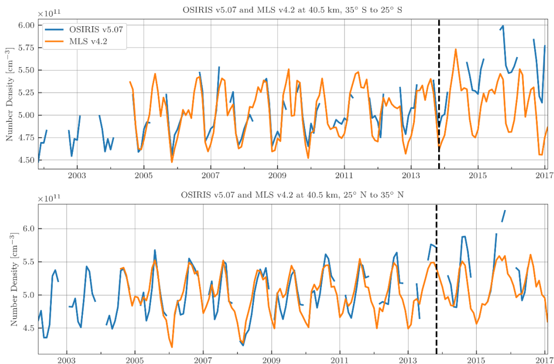
5 Figure 1: OSIRIS version 5.07 and MLS version 4.2 ozone density at 40.5 km and 35 S to 25 S (top), and 25 N to 35 N (bottom). The end of the OSIRIS data set used in the Bourassa et al., 2014 trend study is marked with the vertical black dashed line.
