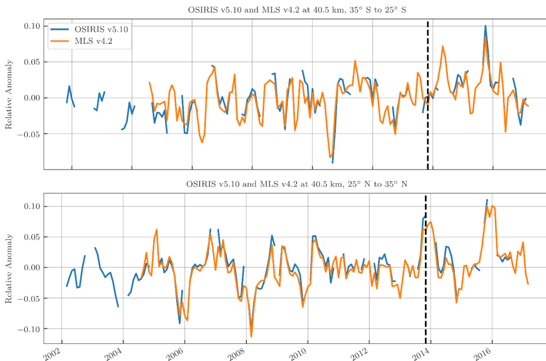
Figure 6: Ozone anomalies used for the trend calculation from pointing corrected OSIRIS version 5.10, together with the same from MLS at the same locations specified in Figure 1.
