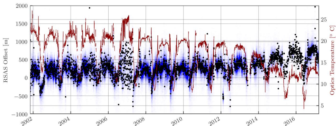
10 Figure 2: Calculated RSAS tangent height offset for every OSIRIS scan (transparent blue dots) and daily averages (black dots). The daily average OSIRIS optics box temperature is shown as the red line.
