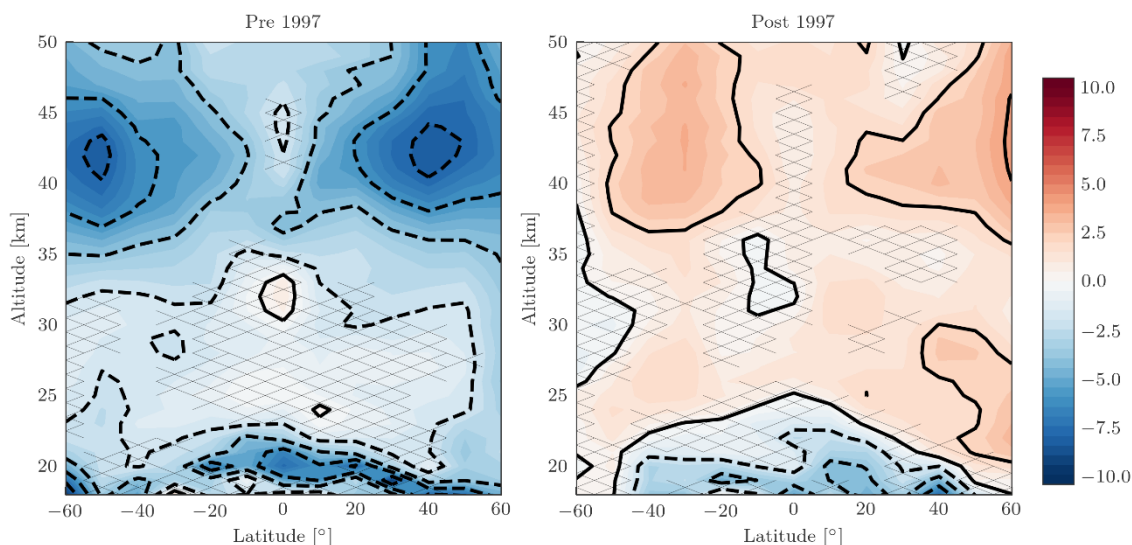
Figure 7: Updated linear ozone trends pre- and post-1997, in percent per decade, following the method of Bourassa et al., 2014, using SAGE II version 7 and the pointing corrected OSIRIS version 5.10 ozone product. The cross-hatching denotes regions that are not statistically significant. Black contours mark steps of 2% per decade.
