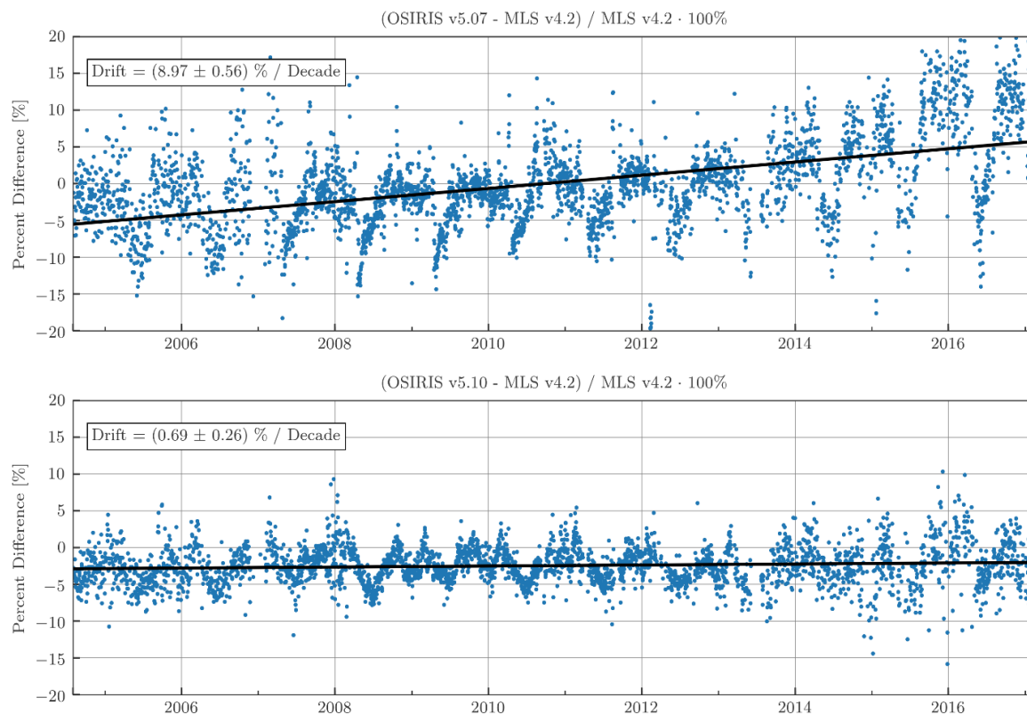
Figure 5: Daily averaged percent difference in zonal mean ozone from 10° S to 10° N at 40.5 km relative to MLS v4.2 for OSIRIS v5.07 (top) and OSIRIS v5.10 (bottom). The MLS v4.2 data is converted to number density on an altitude grid using ERA interim reanalysis pressure and temperature fields. Simple best fit straight line drift estimates are shown in black with uncertainties reported as the 2\sigma values.
