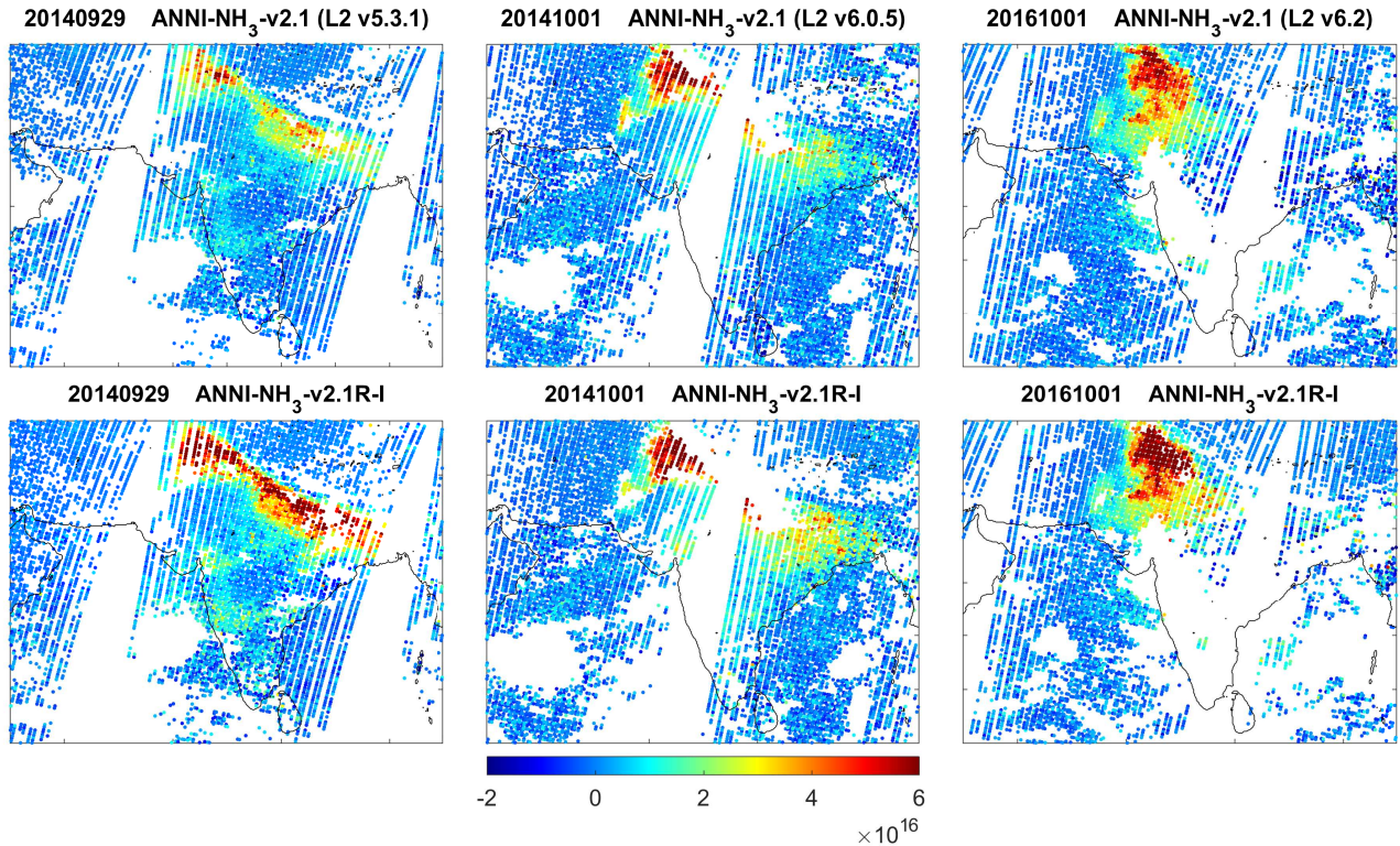
Figure 4. Example retrievals of the morning \text{NH}_3 column ( \text{molec.cm}^{-2} ) over South Asia for the reanalysed retrieval (ANNI- \text{NH}_3 -v2.1R-I, bottom) versus the standard near-real time retrieval (ANNI- \text{NH}_3 -v2.1, top) on 29 September 2014 (input data from Eumetsat L2 v5.3.1), 1 October 2014 (L2 v6.0) and 1 October 2016 (L2 v6.2).
