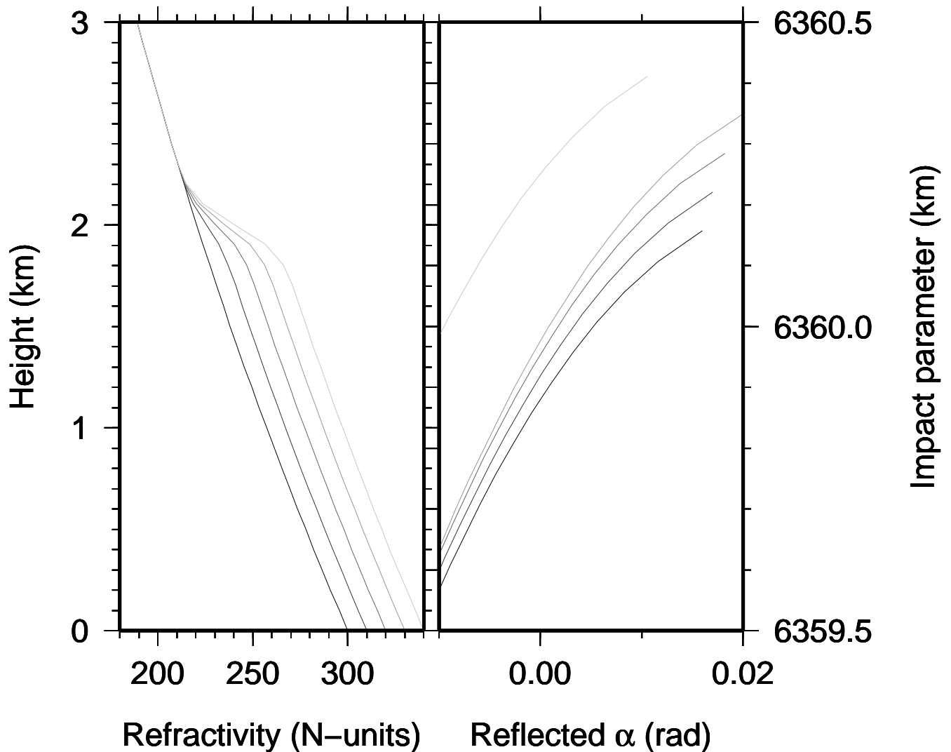
Figure 12. Synthetic case to demonstrate sensitivity of reflection under ducting. The left panel shows a family of synthetic atmospheric refractivity profiles, generated as an exponential function, intended to represent a smooth profile, with a more refractive lower layer, troposphere. The transition is modeled as an error-function. The transition to this extra refraction is sharp very steep, which is common in superrefractive or ducting layers. The right panel shows the corresponding series of reflected bending and impact parameters ( see the lower pannel of Figure 10 for a case with real data ), as evaluated by Equation (3), and indicates that the profile of reflected bending is sensitive to the amplitude of refractivity step across the extra-layer transition.
