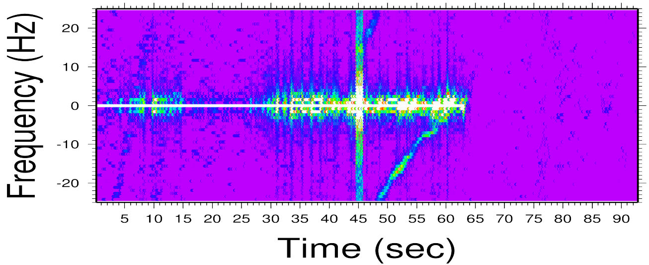
Figure 2. Example radiohologram of deseending-setting COSMIC occultation C001.2011.219.10.43.G15, which presents a reflection. The main signal has been nearly stopped by beating it against a filtered reference. Both components have a narrow spectral width, but the supplementary tone also shows aliasing and-winding (at 46-48 s, +20 Hz). Both tones finally merge. This final section, where the low troposphere is being scanned, shows spectral broadening in both the direct and reflected signals.
