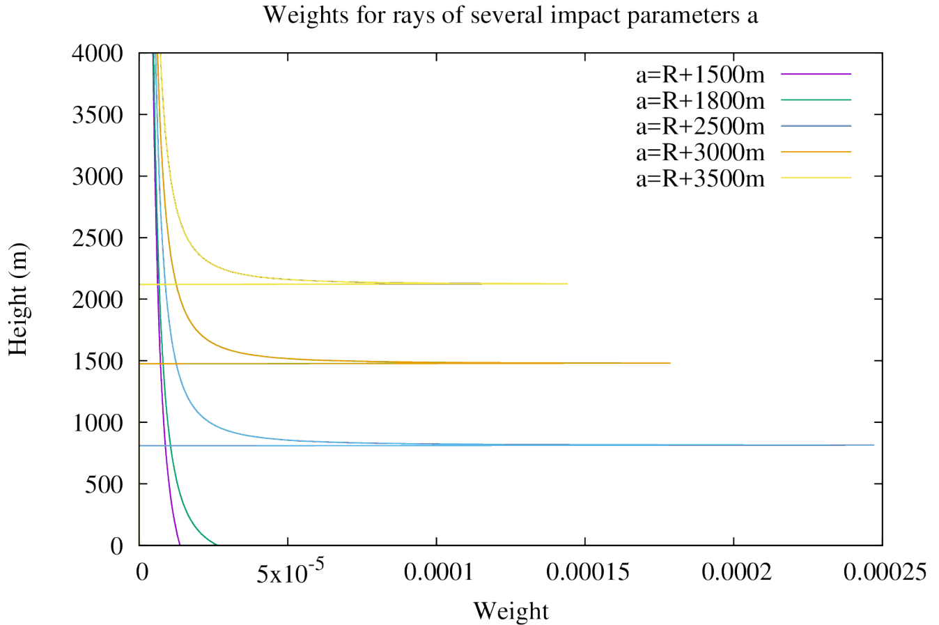
Figure 11. Kernel weight dependency (adimensional) dependence of several paths, with respect to the local refractivity properties of the profile. Three direct paths are shown, those with larger impact parameter ( a = R + 2500m, R + 3000m, R + 3500m ). They all present a sharp peak, providing information that is very independent from each other, and thus high vertical resolution . Two reflected paths are shown, those with smaller impact parameter ( a = R + 1500m, R + 1800m ), which do not show any peak. They provide information that is different between them, but much less independent vertically . With the refractivity profile used, the apparent horizon was approximately located at a_S = R + 1900m .
