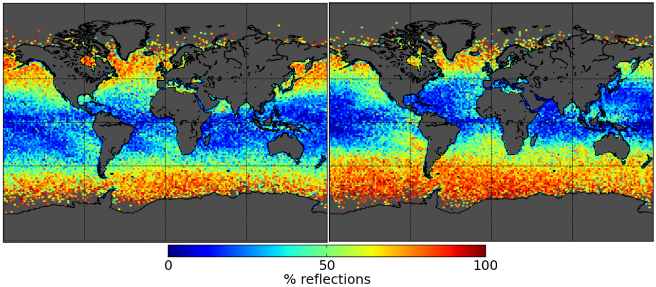
Figure 4. Statistics of GPSRO events identified as showing a reflection, over the ocean, obtained with the COSMIC constellation from 2006 to 2015. Percentage is shown during January and February (left), and during July and August (right). Note that the color scale is different from Figure 3. When the number of events per pixel is too small to derive sensible statistics, these are not shown. In polar oceans, reflections are also very frequent (see also Figure 7). See also Supplementary Movie 2, which shows the seasonal cycle of the median SVM output value over ocean.
