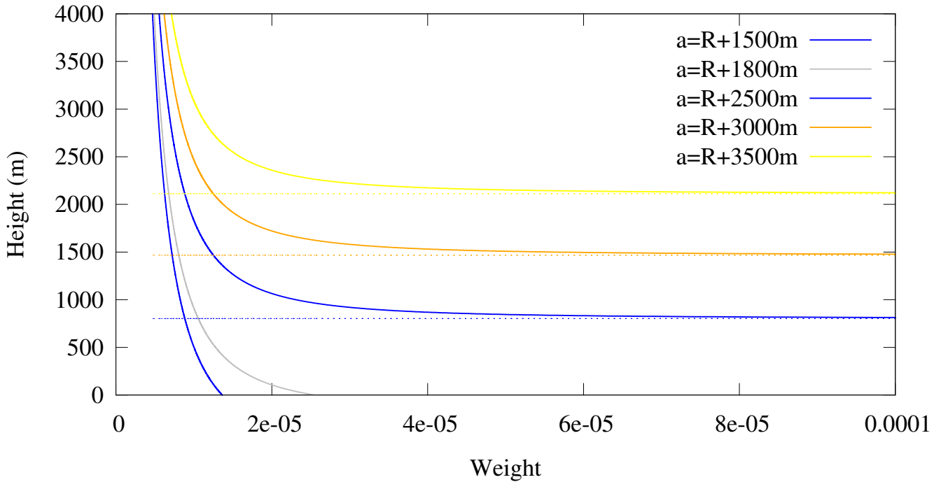
Figure 11. Kernel weight (adimensional) dependence of several paths, with respect to the local refractivity properties of the profile. Weights for three direct paths are shown, with impact parameters ( a = R + 2500m, R + 3000m, R + 3500m ). These kernels present an asymptote (shown dotted, an integrable singularity), and are zero below the asymptote. Given the concentrated weight near the respective asymptote, the information provided by each observation is very independent from each other, leading to an ensemble that provides information of high vertical resolution. Weights for two reflected paths are also shown, with smaller impact parameters ( a = R + 1500m, R + 1800m ). These do not show any narrow concentration of weight. They provide information that is different between them, but much less independent vertically. With the refractivity profile used, the apparent horizon was approximately located at a_S = R + 1900m .
