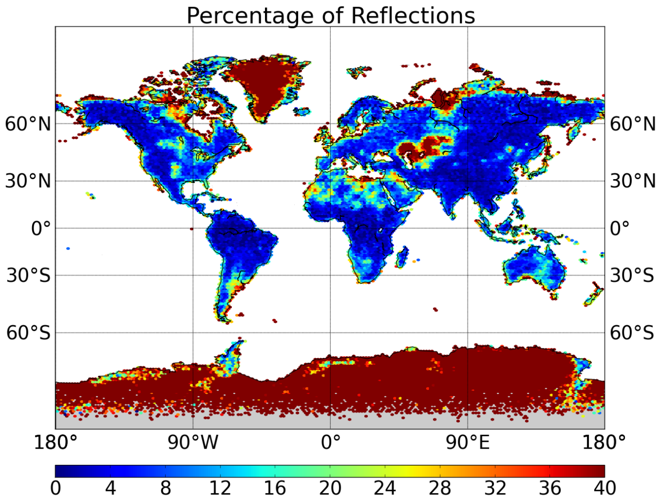
Figure 3. Map of percentage of GPSRO events identified as showing a reflection, over land. The map was compiled with \sim 1,320,000 land events. Reflection events, here identified as those presenting SVM > 0.25 , mostly occur over smooth terrain, free of thick vegetation (deserts, tundra, grasslands), and over continental ice. The largest percentages are found over the ice sheets. The color scale is saturated at 40%. See also Supplementary Movie 1, which shows the seasonal cycle of the median SVM output value over land.
