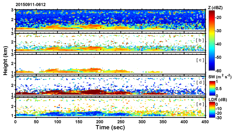
Fig. 1. Figure A1: HTI plot of cloud radar measured (a) Reflectivity (Z), (b) noise removed Z, (c) TEST filtered Z, (d) Spectral Width (SW), and (e) LDR at 0612 UT on 11 Sep 2015.
