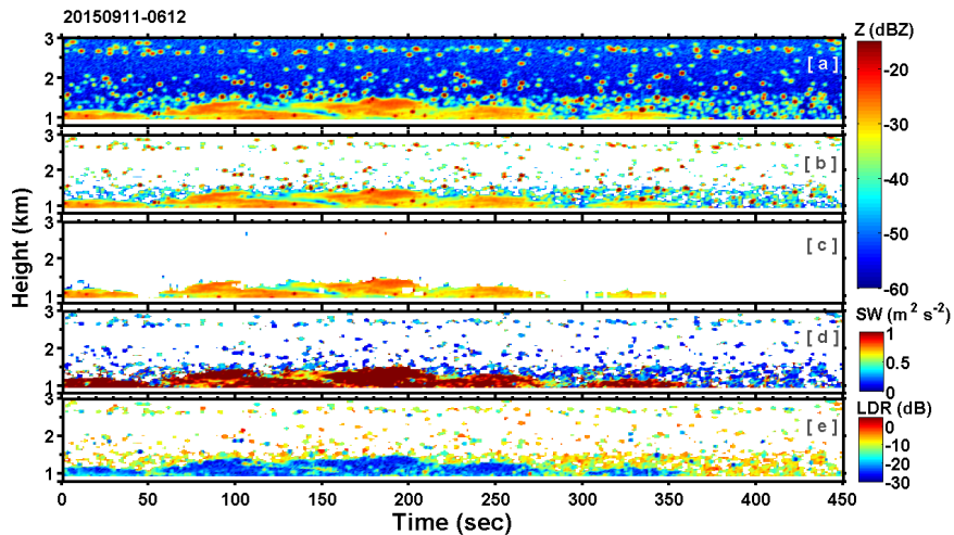
Fig. 1. Figure A1: HTI plot of cloud radar measured (a) Reflectivity (Z), (b) noise removed Z, (c) TEST filtered Z, (d) Spectral Width (SW), and (e) LDR at 0612 UT on 11 Sep 2015.
