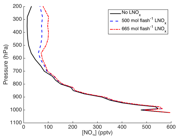
Figure 1. Domain-wide mean WRF-Chem \text{NO}_2 profiles.
