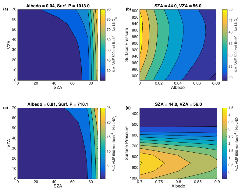
Figure 2. Contour plots of the percent change in the AMF when changing from the mean profile without lightning \text{NO}_x to the mean with lightning \text{NO}_x (500 mol flash ^{-1} ), averaged over the whole WRF-Chem domain. The differences are averaged over all values of RAA. In each plot, two parameters are varied while the other two are held constant. The values of the constant parameters are given above each plot. (a) and (b) use a range of albedos and surface pressure representative of clear pixels; (c) and (d) for cloudy pixels.
