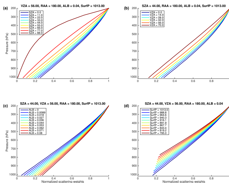
Figure 3. Vectors of scattering weights and their variation with each of the four most important look-up table input parameters. Values are representative of clear-sky conditions. Each scattering weight vector is scaled so that the top most entry is 1. Scattering weights are only shown above the surface pressure.
