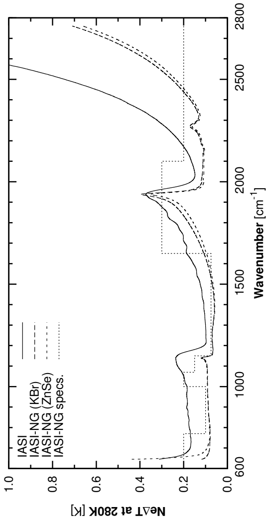
Figure 1. NedT noise at 280 K for IASI and IASI-NG (source data from E. Pequignot, CNES)
