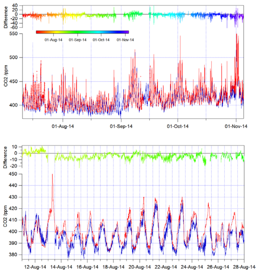
Figure 9. Open path (blue), in situ (red) and difference (OP – in situ, black coloured by time) measurements of CO 2 . All raw OP data have been reduced by a factor of 1.025 (~ 10 ppm) to remove measurement bias relative to the in situ data. In the corrected data, there is zero bias for wind speeds > 6 m s -1 over the entire measurement period (see text for detail). (a) shows the whole measurement period. (b) illustrates a selected period with a consistent, real OP-in situ difference relative to the well mixed average.
