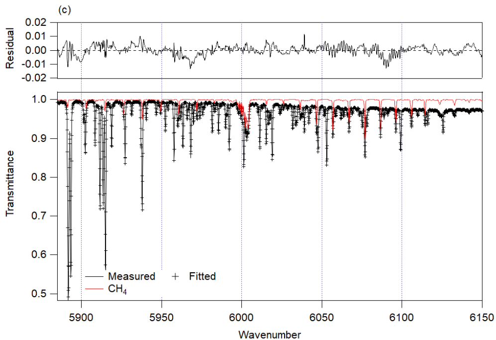
Figure 4. Typical fits for (a) \text{O}_2 band centred near 7880 \text{ cm}^{-1} (b) \text{CO}_2 bands centred near 4850 and 4980 \text{ cm}^{-1} and (c) \text{CH}_4 band centred near 6000 \text{ cm}^{-1} . In each plot the target species is in red, and the remaining absorption is dominated by water vapour. See Table 1 for details of all interfering and co-fitted species.
