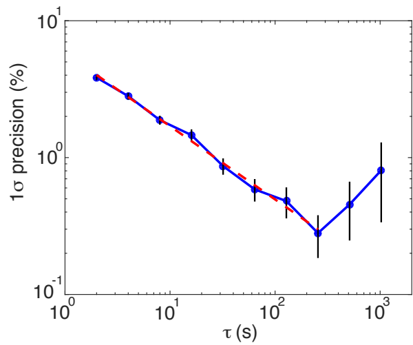
Figure 7: Normalized Allan-Werle deviation as a function of averaging time ( \tau ) demonstrates the precision benefit of time-averaging up to 250 s. Fitting the data with \tau < 250 s yields a slope of -0.5 (dashed red line), consistent with white noise dominating the variability at shorter averaging periods. [HCHO] = 5 ppbv.
