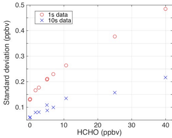
Figure 6: The standard deviation as a function of HCHO is shown to demonstrate the precision of the HCHO measurement for 1 s and 10 s averaging.
