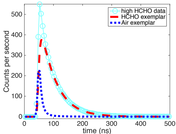
10 Figure 4: Exemplar time profiles are obtained in the laboratory. The air exemplar is created by averaging the profile with no added HCHO (blue dashed line), and the HCHO exemplar (red dashed line) is obtained by subtracting the air exemplar from data with high (29 ppbv) HCHO (cyan circles).
