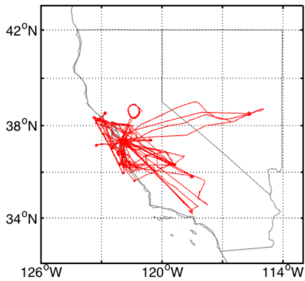
10 Figure 11: Map of AJAX flight tracks with COFFEE in payload through March 2017.
