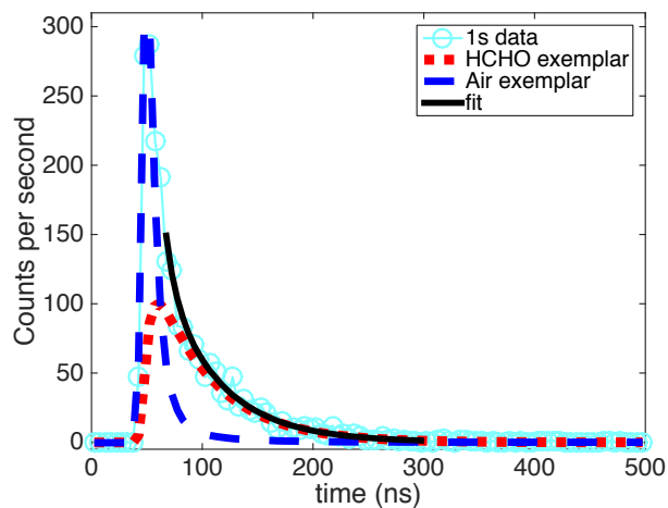
15 Figure 5: Each 1s data profile (cyan circles) is fit using a linear combination of the air (dashed blue line) and HCHO (dashed red line). The fit profile, over the time window used for the least squares fit, is shown in black. HCHO mixing ratio is 8 ppbv.
