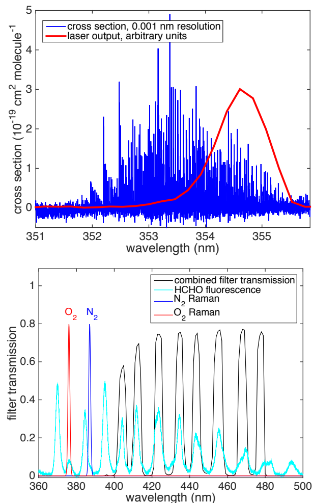
15 Figure 1: Top Panel: The HCHO absorption spectrum (Co et al., 2005), averaged to 0.001 nm resolution, and the excitation laser spectrum are shown. Bottom Panel: The optical filter transmission spectrum is shown for the detection axis 2 (multi-band pass filter). The HCHO fluorescence and the N 2 and O 2 Raman spectra are included for reference, all with arbitrary units.
