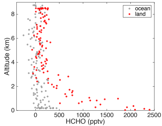
Figure 12: Flight data for AJAX Flight 185 on 2016 April 19. Top Panel: time series of HCHO (10 s data, blue) and the corresponding aircraft altitude (black), with spiral profiles over land (red) and ocean (gray) highlighted. Bottom Panel: altitude profiles of HCHO (10 s data) over land (red) and ocean (gray).
