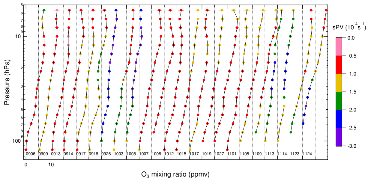
Figure 3. Time series of DIAL O 3 profiles at the OAPA site. Each profile is shifted 5 ppmv. Data are color-scaled based on sPV values. Observation dates in 2009 are shown as MMDD, e.g., 0906 is September 6, 2009.
