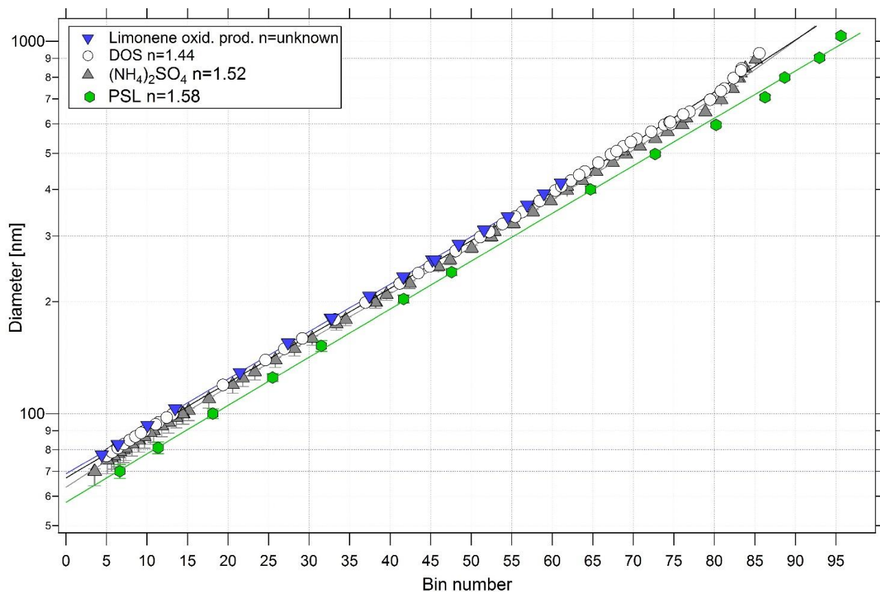
Fig.3. Calibration particle diameter as a function of UHSAS-2 (not thermodenuded) bin number for particles composed of PSL, (\text{NH}_4)_2\text{SO}_4 , DOS and limonene ozonolysis products. Uncertainties are shown for (\text{NH}_4)_2\text{SO}_4 and PSL but are often obscured by the symbols.
