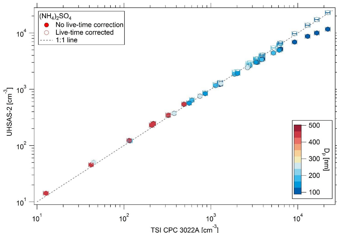
Fig.5. Relationship between the UHSAS-2 and the CPC particle number concentration ( \text{cm}^{-3} ) for nearly monodisperse (\text{NH}_4)_2\text{SO}_4 aerosol of various sizes ( >0.1 \mu\text{m} ) at ambient pressure. Dashed line represents 1:1 correspondence line.
