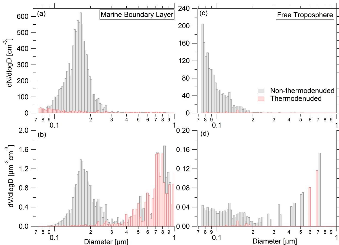
Fig.11. Example of an averaged dry aerosol size distribution from UHSAS-1-TD and UHSAS-2 as sampled in the MBL (21.74° N, 1080 hPa) showing (a) number and (b) volume; and for a separate size distribution sampled in the FT (3.4° N, 293 hPa) showing (c) number and (d) volume. For particles with D_p between 0.1 and 0.9 \mu\text{m} , in the MBL case ((a), (b)) 94 % of the total number and 54 % of the total volume volatilized in the thermodenuder, while in the FT case ((c), (d)) 94 % of the number and 76 % of the volume volatilized.
