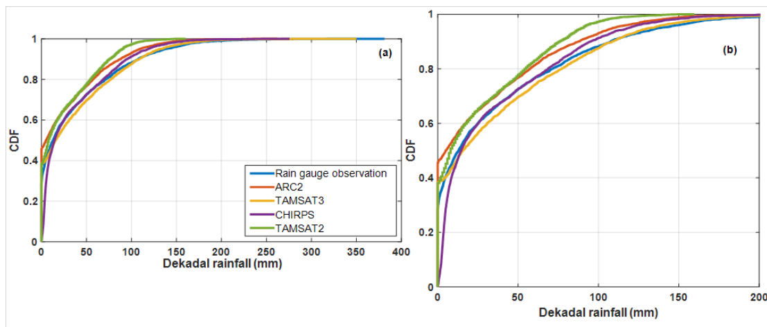
Fig. 2. Cumulative distribution function (CDF) of dekadal rainfall for ground rainfall observation, ARC 2, TAMSAT, and CHIRPS rainfall estimates (a) and magnified view of their CDF for 0 to 200 mm part (b) ov
