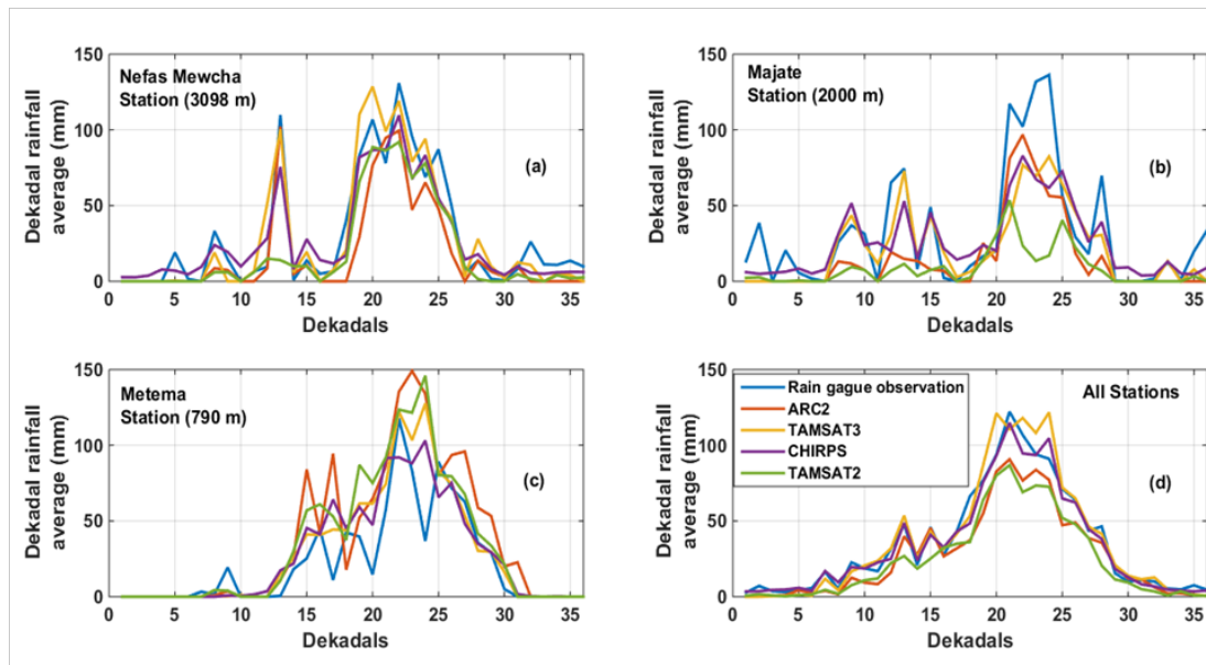
Fig. 3. Comparison of the satellite rainfall products at rain gauge stations with wider difference in elevation values (e.g., > 2000m) based on dekadal average for over the Upper Blue Nile basin for the perio
