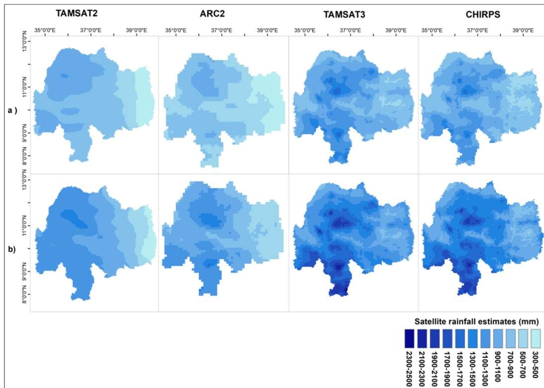
Fig. 1. Comparison of mean satellite rainfall estimates for: (a) Kiremt season (June-September), and (b) annual rainfall over the Upper Blue Nile basin for the period of 2000-2015. Years with missed
