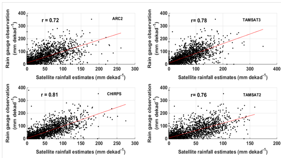
Fig. 5. plot between rain gauge observations and satellite rainfall estimates at dekadal temporal scale over the Upper Blue Nile basin for the period of 2000-2015.
