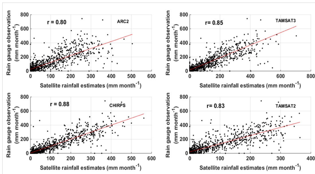
Fig. 4. Scatter plot between rain gauge observations and satellite rainfall estimates at monthly temporal scale over the Upper Blue Nile basin for the period of 2000-2015
