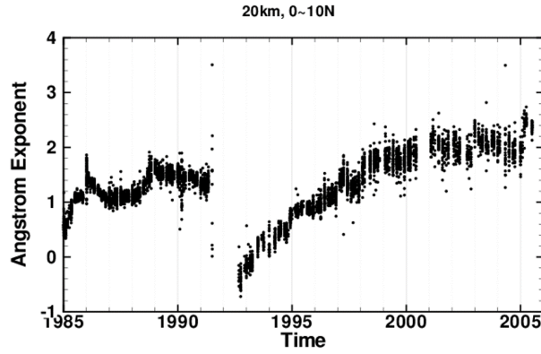
Figure 7. Angstrom exponent \alpha(525/1020) derived from SAGE II SOT measurements during its measurement history. This picture corresponds to measurements at altitude 20 km for the 0 - 10^\circ North latitude bin. Cases for which the measured aerosol extinction at 1020 nm < 4 \times 10^{-6} km were excluded from this analysis [L. Thomason, private communication].
