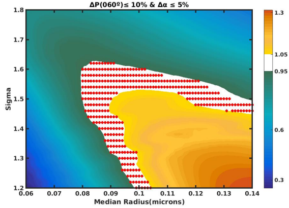
Figure 21. The background contour plot is the same as in Fig. 20. This time, red circles appear only for cases in which the Angstrom coefficient ratio is within \pm 5\% of 1 and the aerosol phase function is within \pm 10\% of the V1 aerosol size distribution value at \Theta = 60^\circ . Nearly every aerosol size distribution that satisfies the Angstrom coefficient ratio criterion also satisfies the aerosol phase function criterion for this case.
