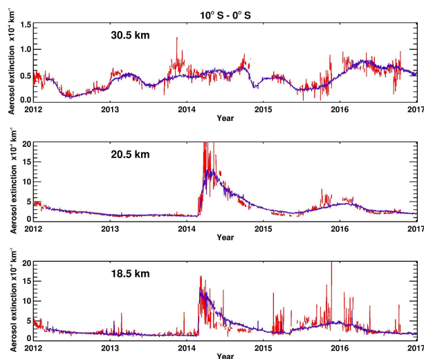
Figure 24. OMPS LP V1 (blue line) and OSIRIS V5.07 (red line) retrieved aerosol extinction daily zonal means at selected altitudes from 2012 to 2016, at latitudes between 10^\circ S and 0^\circ S. The OSIRIS data set reports aerosol extinction at 750 nm, so the OMPS aerosol extinction was converted from 674 nm to 750 nm by using the angstrom coefficient consistent with the aerosol size distribution assumed in the OMPS LP V1 algorithm.
