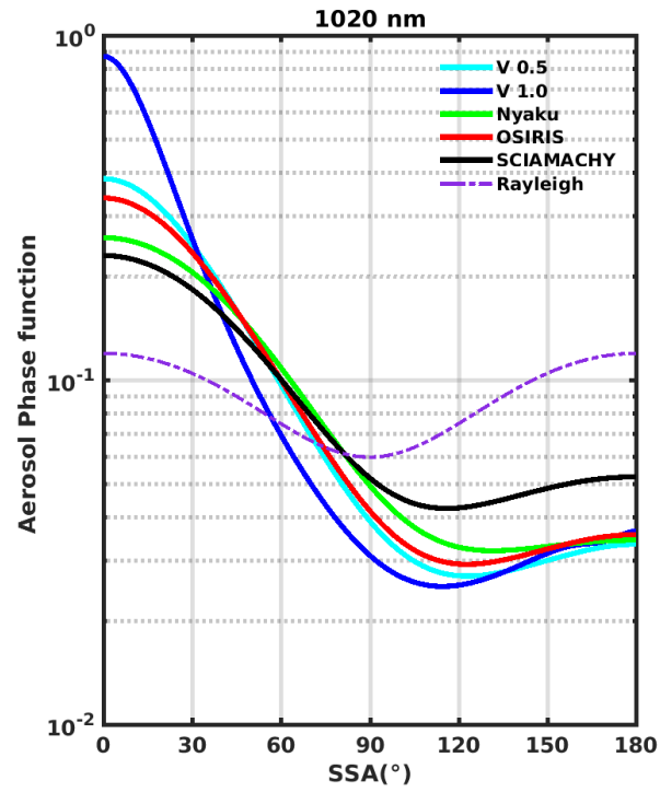
Figure 12. The aerosol phase function at 1020 nm as a function of SSA (or \Theta ) for the aerosol size distributions listed in Tables 1 - 2.
