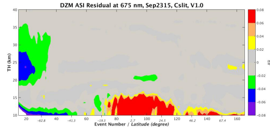
Figure 19. Daily zonal mean aerosol scattering index ( ASI , or y ) residuals for center slit observations on September 23, 2015 (derived from the y measurements shown in Fig. 16).
