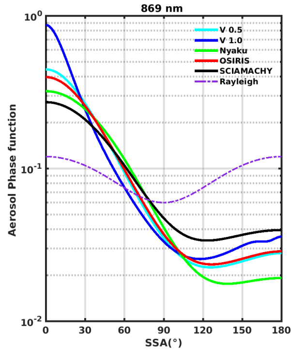
Figure 11. The aerosol phase function at 869 nm as a function of SSA (or \Theta ) for the aerosol size distributions listed in Tables 1 - 2.
