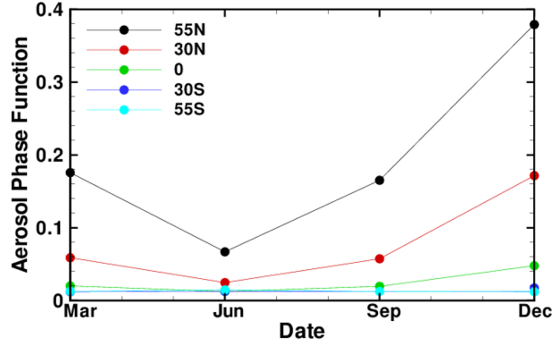
Figure 4. The seasonal variation of the aerosol phase function at several latitudes for the SNPP OMPS LP orbit. The aerosol size distribution described in Table 1 for the V1 aerosol extinction retrieval algorithm is assumed.
