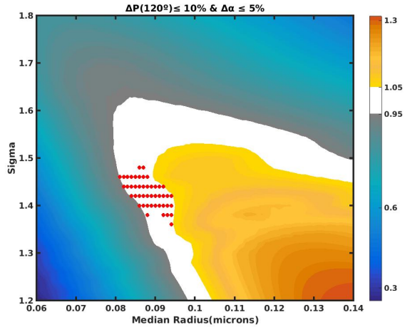
Figure 22. Identical to Fig. 21, except that the aerosol phase function comparison is done for \Theta = 120^\circ . For this viewing geometry, the aerosol phase function criterion is much more useful in determining the aerosol size distribution properties: Note the smaller number of red circles (relative to Fig. 21), centered around the true values of r_1 (0.09 \mu\text{m}) and \sigma_1 (1.4) .
