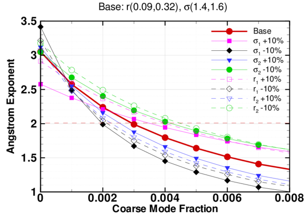
Figure 8. Variation of Angstrom exponent \alpha(525/1020) with aerosol properties for the V1 OMPS LP aerosol extinction retrieval algorithm characteristics. Each curve shows the variation of (\alpha(525/1020)) with f_c for a given set of median radii and mode widths. In addition to the “base” curve (which uses the V1 characteristics listed in Table 1), several curves show how the value of \alpha(525/1020) changes as the values of (r_1, \sigma_1, r_2, \sigma_2) in Table 1 are perturbed by \pm 10\% .
