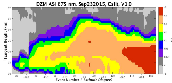
Figure 16. Daily zonal mean aerosol scattering index ( ASI , or y ) measured by the SNPP OMPS LP instrument. This picture corresponds to center slit observations on September 23, 2015. The x-axis is labeled with both the event number (solid) and tangent point latitude (italics). The color scale is non-linear, designed to highlight relatively small y values in the SH.
