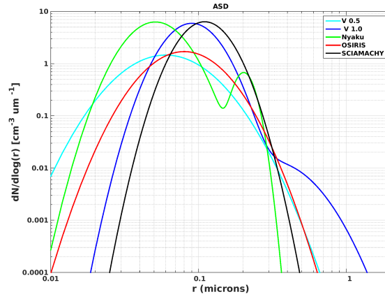
Figure 6. Illustration of the aerosol size distributions used in several recent LS aerosol extinction retrieval algorithms, including OSIRIS (V5), SCIAMACHY (V1.1), and OMPS (V0.5 and V1). The aerosol size distribution studied by (Nyaku, 2016) is also represented.
