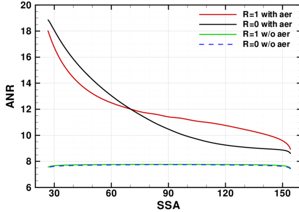
Figure 14. Altitude normalized radiances ( ANR , or \rho ) at 675 nm as a function of SSA (or \Theta ) under aerosol-free and aerosol conditions, with both non-reflecting ( R = 0 ) and perfectly-reflecting ( R = 1 ) surface conditions. The values of h and h_n are 25.5 and 40.5 km, respectively.
