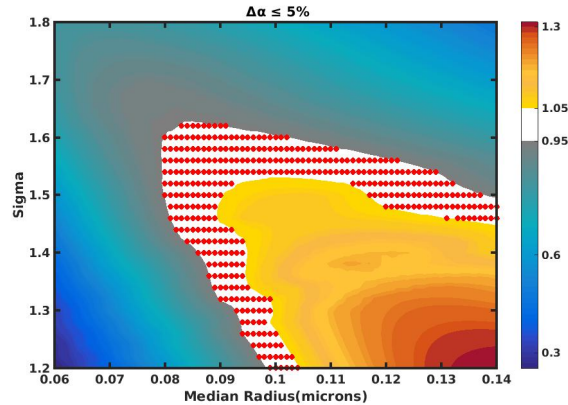
Figure 20. Contour plot showing the ratio of the Angstrom coefficient \alpha for a given aerosol size distribution to the V1 aerosol size distribution \alpha \approx 2 . Cases for which this ratio is within \pm 5\% of 1 are highlighted in white. The coarse mode properties are fixed in this example at the V1 aerosol size distribution values ( r_2 = 0.32\mu\text{ m} , \sigma_2 = 1.6 ), while the fine mode properties vary in the vicinity of the V1 aerosol size distribution values ( r_1 = 0.09\mu\text{ m} , \sigma_1 = 1.4 ). Red circles indicate the individual cases calculated to create this figure.
