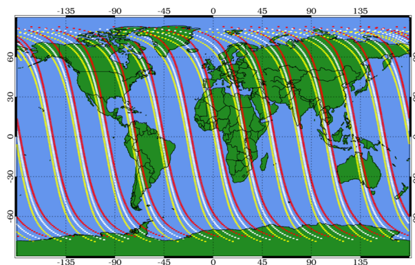
Figure 1. Daily coverage provided by the OMPS LP instrument mounted on the SNPP satellite. The tangent point for the LOS corresponding to each observation is indicated, with red, white and yellow circles depicting the left, center and right slit observations.
