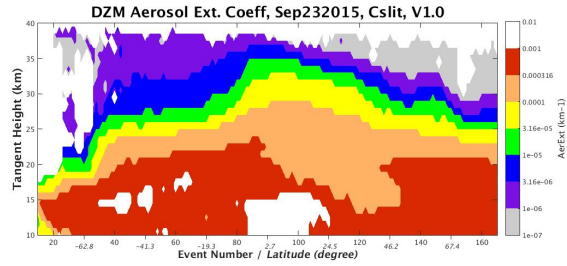
Figure 18. Daily zonal mean aerosol extinction for center slit observations on September 23, 2015 (derived from the y measurements shown in Fig. 16).
