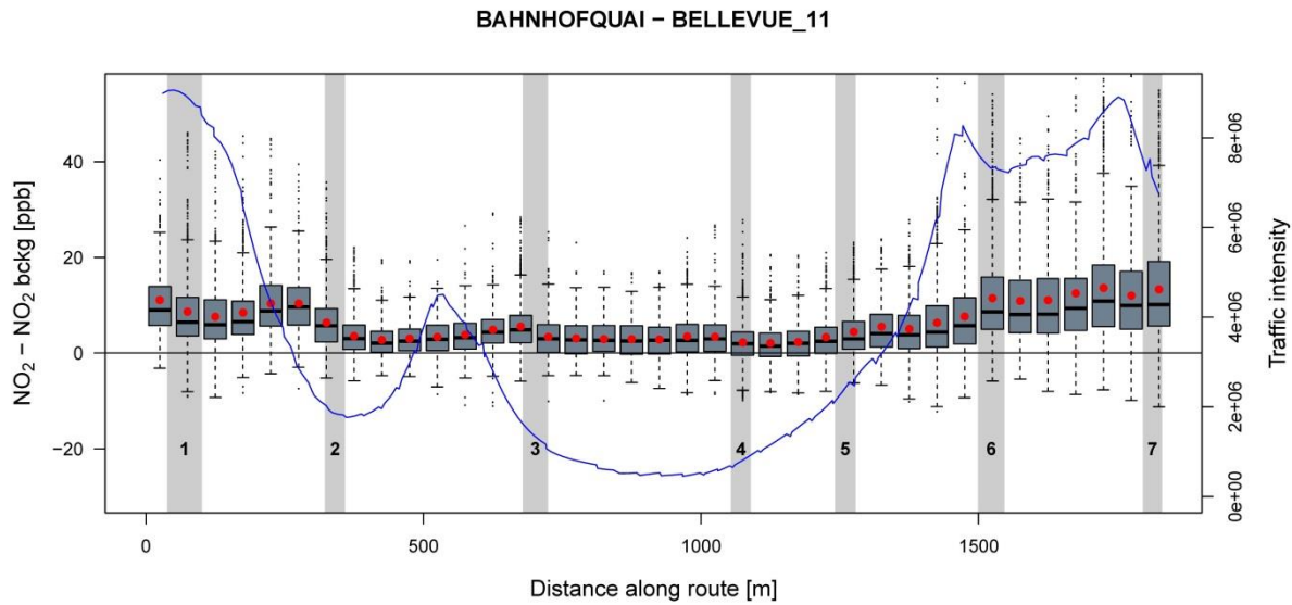
Figure 11: Estimated local emission signal (i.e. difference between measured \text{NO}_2 and background \text{NO}_2 ) between stations Bahnhofquai (1) and Bellevue (7) aggregated by 50 m track length. The traffic intensity is indicated by the blue line.
