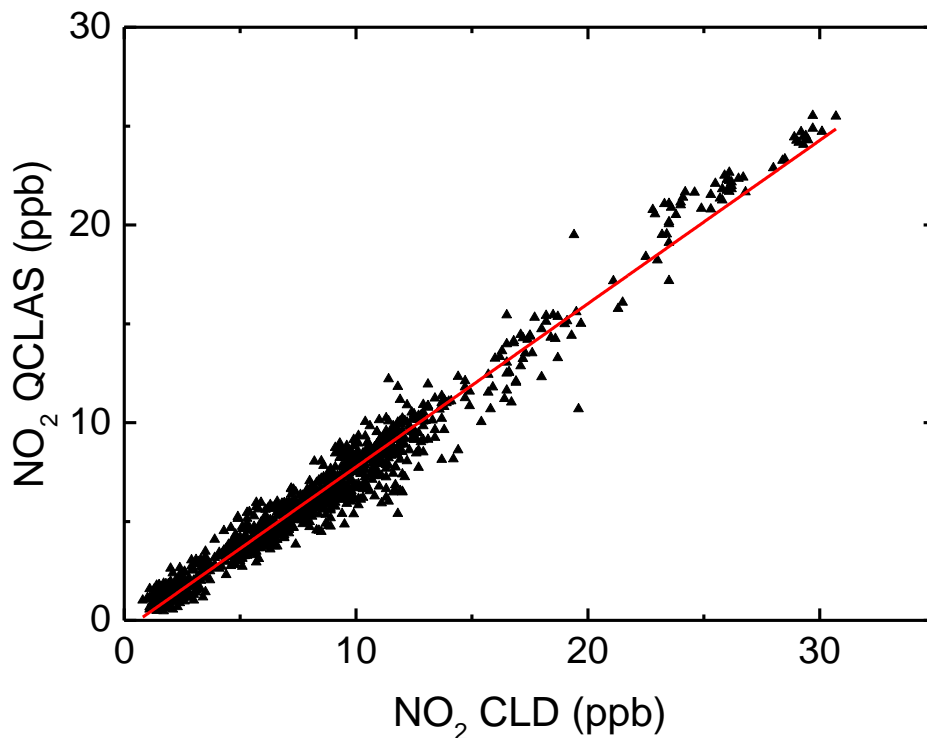
Figure 6: Scatter plot of QCLAS concentration measurements (1 minute means) versus CLD measurements (1 minute means). Both instruments ran in parallel at the AQM site in Duebendorf, Switzerland, in the period 17 Jun 2015 to 19 Jun 2015. The red line is a linear fit to the data with slope 0.83 \pm 0.004 , intersect -0.49 \pm 0.04 and an R^2 of 0.985.
