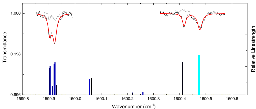
Figure 2: Transmission spectra recorded by the instrument: Zero-air (grey) and 49 ppb of NO 2 (black) both with 0.5 % water. The red line represents the least-square fit of the 49 ppb NO 2 spectrum. The dark-blue bars indicate the line-strength of NO 2 absorption lines and the light-blue bar indicates a water line.
