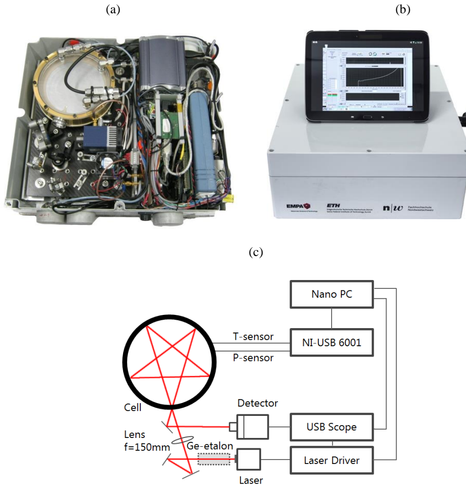
Figure 1: (a, b) Photograph of the QCLAS instrument with the top cover removed and in the final layout. The overall weight is 10 kg and it operates on 12V DC. (c) Schematic of the instrument with the key optical and hardware elements.
