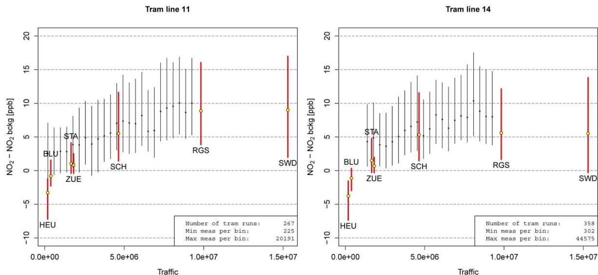
Figure 12: Local emission signal (i.e. difference between NO 2 measurements and the background concentration signal) related to the traffic intensity. The values from the tram instrument are aggregated by equally spaced bins and depicted in black. The values from the AQM sites are shown in red. The lines span the 25% to the 75% quantiles, the dots represent the 50% quantile.
