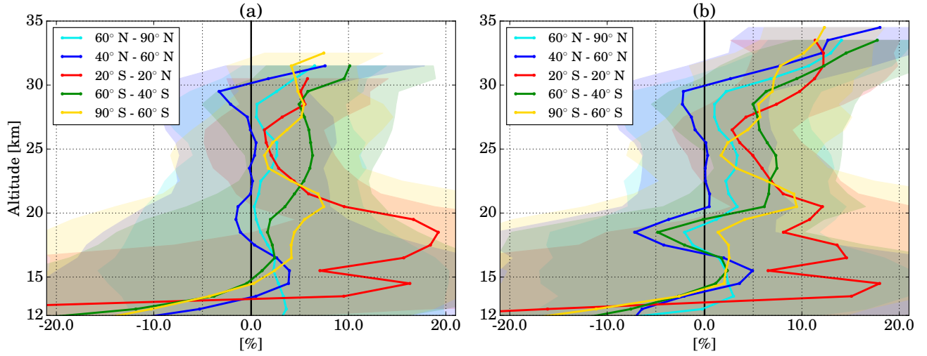
Figure 10. Relative differences between collocated IUP-OMPS profiles and ozonesonde measurements in five latitudinal bands ( 60^\circ N– 90^\circ N, 40^\circ N– 60^\circ N, 20^\circ S– 20^\circ N, 60^\circ S– 40^\circ S and 90^\circ S– 60^\circ S), using in panel (a) averaging kernel convolution and in panel (b) vertical averaging. Corresponding standard deviations are shown as shaded areas.
