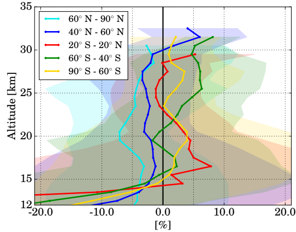
Figure 11. Relative differences between collocated IUP-OMPS profiles and ozonesonde measurements in five latitudinal bands ( 60^\circ N– 90^\circ N, 40^\circ N– 60^\circ N, 20^\circ S– 20^\circ N, 60^\circ S– 40^\circ S and 90^\circ S– 60^\circ S) for the 2013 data set, with corresponding standard deviations as shaded areas.
