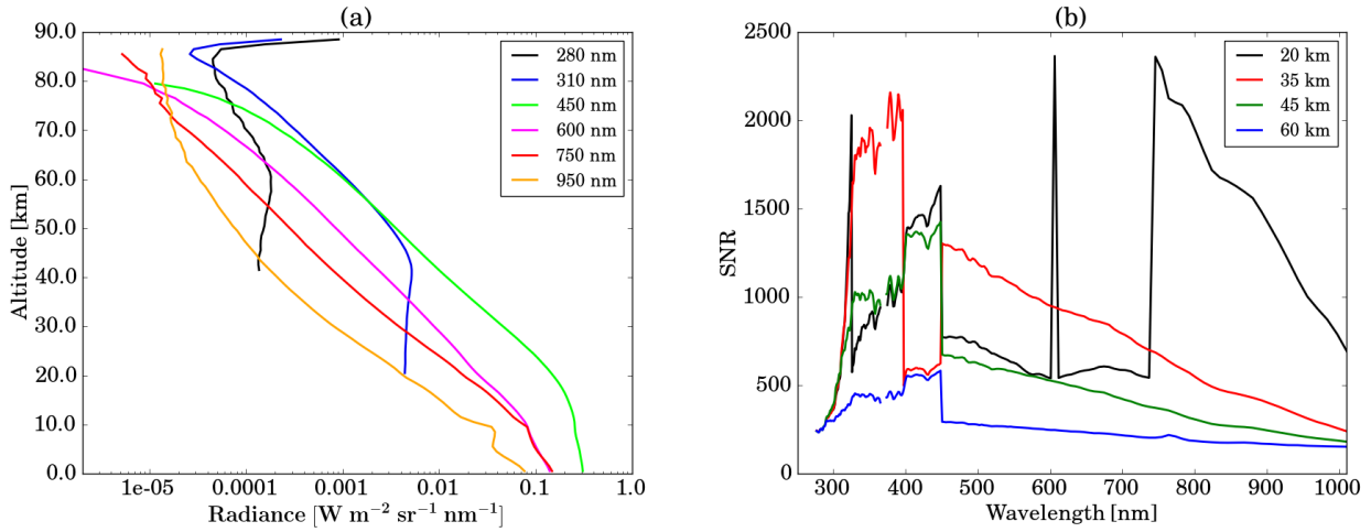
Figure 2. Left panel: example of OMPS-LP radiance profiles at some selected wavelengths; right panel: OMPS-LP signal-to-noise ratio (SNR) at different tangent heights.
