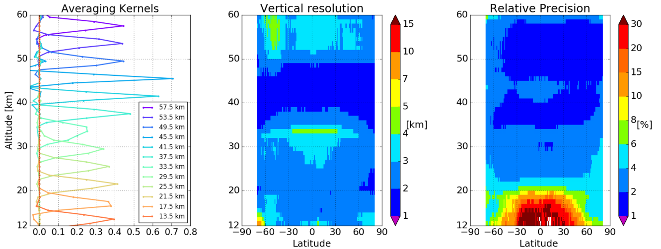
Figure 5. From left to right, examples of averaging kernels (plotted every 4 km for sake of clarity), vertical resolution and theoretical precision of the retrieval scheme. AKs are plotted for a measurement at 30° N, whereas vertical resolution and theoretical precision are shown as a function of latitude, i.e. solar zenith angle, for one day (15 September 2016).
