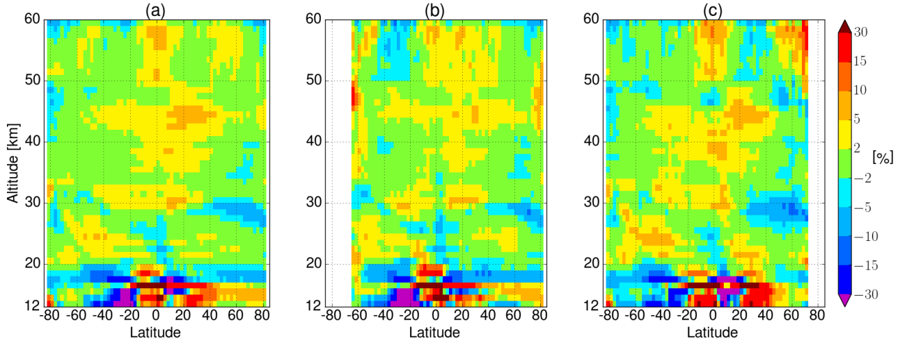
Figure 8. Relative differences (Eq. 9) averaged over 2.5^\circ latitude bins, plotted as a function of altitude. Panel (a) whole year, panel (b) June, July and August, panel (c) January, February and December.
