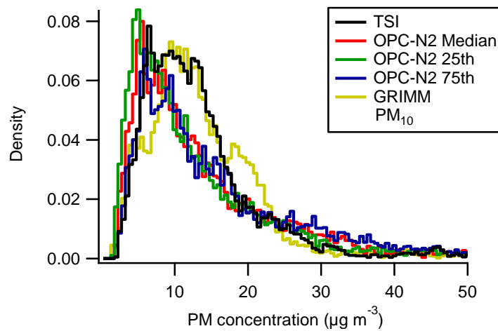
Figure 4: Histogram of measured PM_1 , PM_{2.5} and PM_{10} mass concentrations by the TSI 3330, GRIMM and median and inter-quartile values for the 14 OPC-N2. Note the different x and y axis scales.
