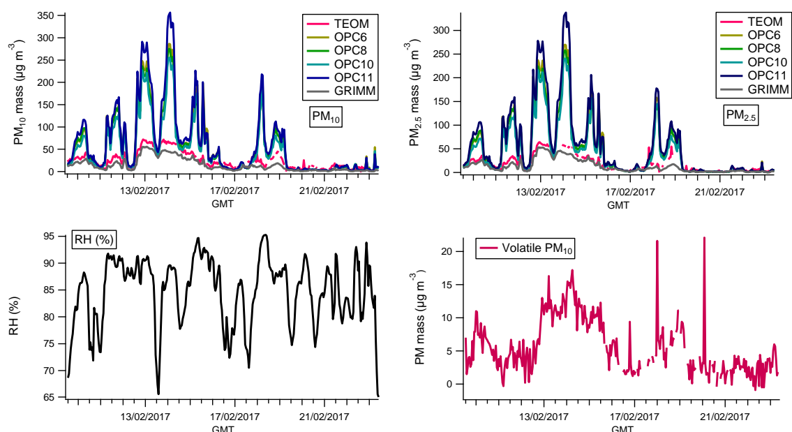
Figure 7: Time series for hourly measured PM mass concentrations by the TEOM, four OPC-N2 and GRIMM at Tyburn Rd urban background AURN station. The volatile particle mass concentration as measured by the TEOM-FDMS and relative humidity measured at Tyburn Rd also shown.”
