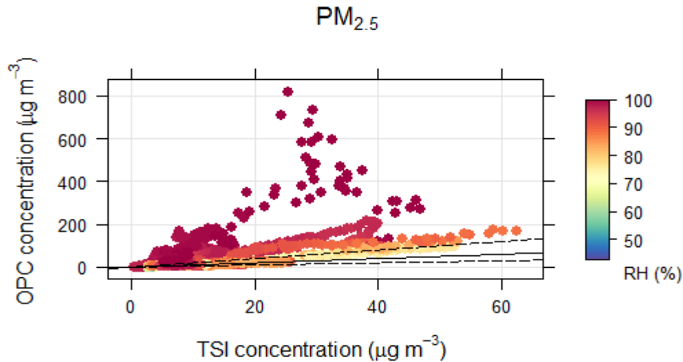
Figure 6: Measured concentrations by the TSI 3330 compared to the median concentration measured by the 14 OPC-N2, coloured by the ambient relative humidity. Also shown are the 1:1 (solid) and 0.5:1 and 2:1 (dashed) lines.
