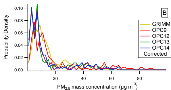
Figure 9: Histogram of measured PM_{2.5} concentrations by the GRIMM PAS 1.108 and the 4 OPC-N2s for January. The uncorrected OPC-N2 concentrations are shown in the left plot (A), while the right plot (B) shows the RH corrected OPC-N2 concentrations.
