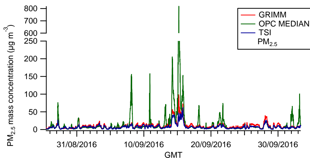
Figure 5: Time series of the measured PM_{2.5} mass concentrations by the TSI, GRIMM and median concentration measured by the 14 OPC-N2 at EROS.
