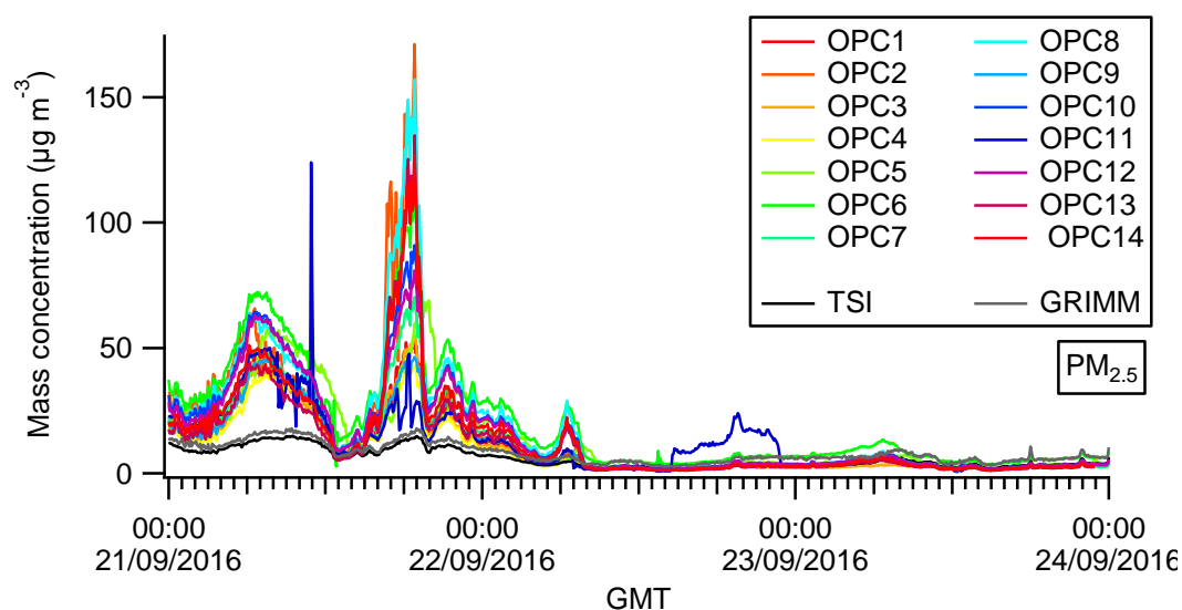
Figure 1: Time series of \text{PM}_{2.5} concentrations measured by all OPC-N2 and the reference instruments, TSI 3330 and GRIMM for selected period with high OPC-N2 data coverage.
