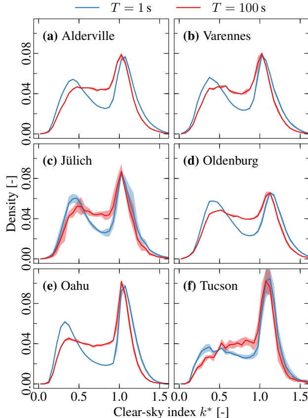
Figure 2. Distributions of clear-sky index k^* under mixed-sky conditions for two averaging times T = 1\text{ s} and T = 100\text{ s} and all six locations, estimated from histograms using a bin width of 0.05. The spread across multiple single-sensor distributions is indicated using semi-transparent coloring, while the solid lines are derived by averaging the single-sensor densities in each bin.
