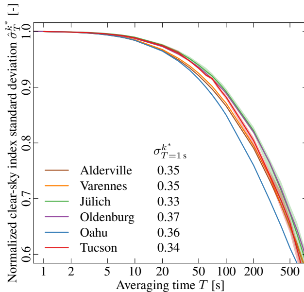
Figure 3. Structures of normalized clear-sky index standard deviation \hat{\sigma}_T^{k^*} as a function of averaging time T under mixed-sky conditions for all six available locations. The normalization factors \sigma_{T=1s}^{k^*} are quoted for each location. The spread across multiple individual single-sensor structures is indicated using semi-transparent coloring, while the solid lines are derived by averaging the single-sensor structures for each T .
