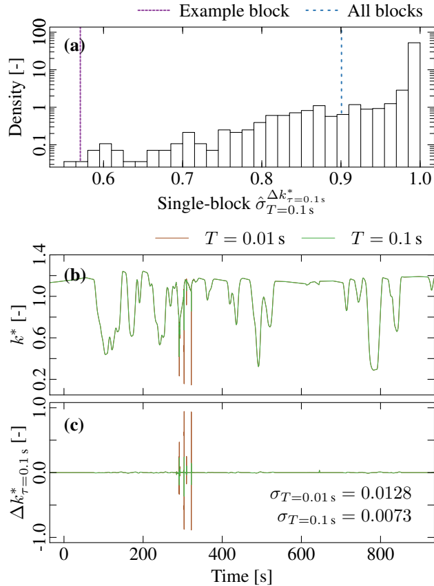
Figure 8. (a) The distribution of all Varennes-based single 900-s-block values of normalized clear-sky index increment standard deviation \hat{\sigma}_{T=0.1s}^{\Delta k_{\tau=0.1s}^*} for T = 0.1 s and \tau = 0.1 s, including an indication of the values corresponding to all blocks (as in Fig. 6) and to an example block featuring a very low \hat{\sigma}_{T=0.1s}^{\Delta k_{\tau=0.1s}^*} = 0.57 . Note the logarithmic scaling of the vertical axis. (b) Clear-sky index k^* time series of the 900 s example block for T = 0.01 s and T = 0.1 s, measured in Varennes on 2016-06-23, starting at 07:41:40 EDT. (c) The corresponding clear-sky index increments \Delta k_{\tau=0.1s}^* for an increment time step \tau = 0.1 s, quoting the values of the respective increment standard deviations.
