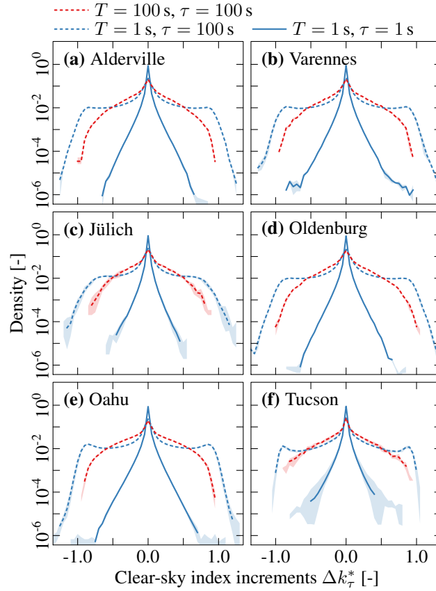
Figure 5. Location-specific distributions of clear-sky index increments \Delta k_\tau^* under mixed-sky conditions for averaging times T = 1 s and T = 100 s, and increment time steps \tau = 100 s and \tau = 1 s, using a bin width of 0.05. The spread across individual single-sensor distributions is indicated using semi-transparent coloring for all bins with data from at least two sensors. The averages of the single-sensor densities are presented as solid or dashed lines for the bins that contain data from every sensor.
