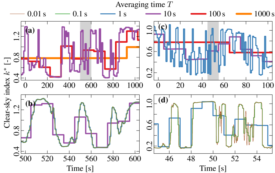
Figure 1. Two examples of highly-variable clear-sky index k^* time series under mixed sky conditions: panels (a,b) show a typical example of a 1000 s period using six averaging times T , namely (a) T = 1000 s, T = 100 s, and T = 10 s, and (b) T = 10 s, T = 1 s, T = 0.1 s, and T = 0.01 s; panels (c,d) show an unusual 100 s example with evident variability down to the shortest time scales with averaging periods (a) T = 100 s, T = 10 s, and T = 1 s, and (b) T = 1 s, T = 0.1 s, and T = 0.01 s. The time series were measured in Varennes on March 2, 2016, starting at 15:01:35 EDT (a,b), and on September 21, 2016, starting at 15:06:35 EDT (c,d). The gray areas in the top row indicate the excerpts presented in the bottom row.
