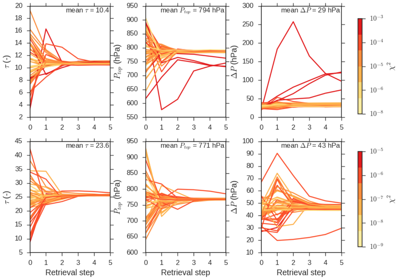
Figure 7 Example iteration in retrieved cloud properties for synthetic micro-window retrievals for test cases with cloud optical depth near 10 (top) and 25 (bottom). Each line represents the iterations through one of the 50 sample retrievals. The lines are coloured according to their \chi^2 values, note the separate colour bars for the top and bottom rows with larger \chi^2 for the top cases.
