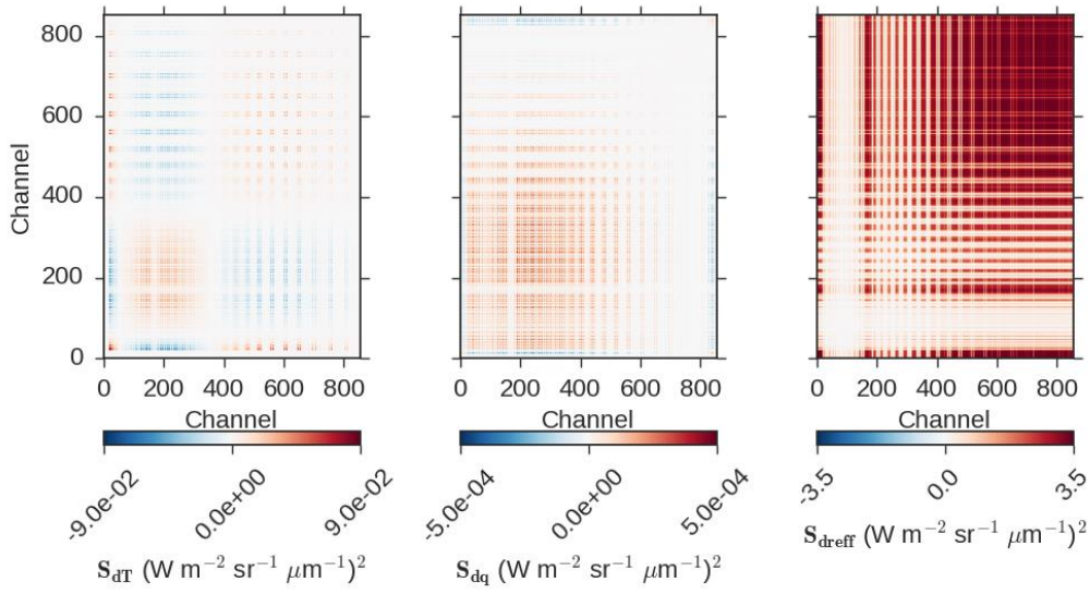
Figure 2 Example covariance matrices for each component as labelled in the colour bar: (left) temperature, (middle) humidity, (right) effective radius.
