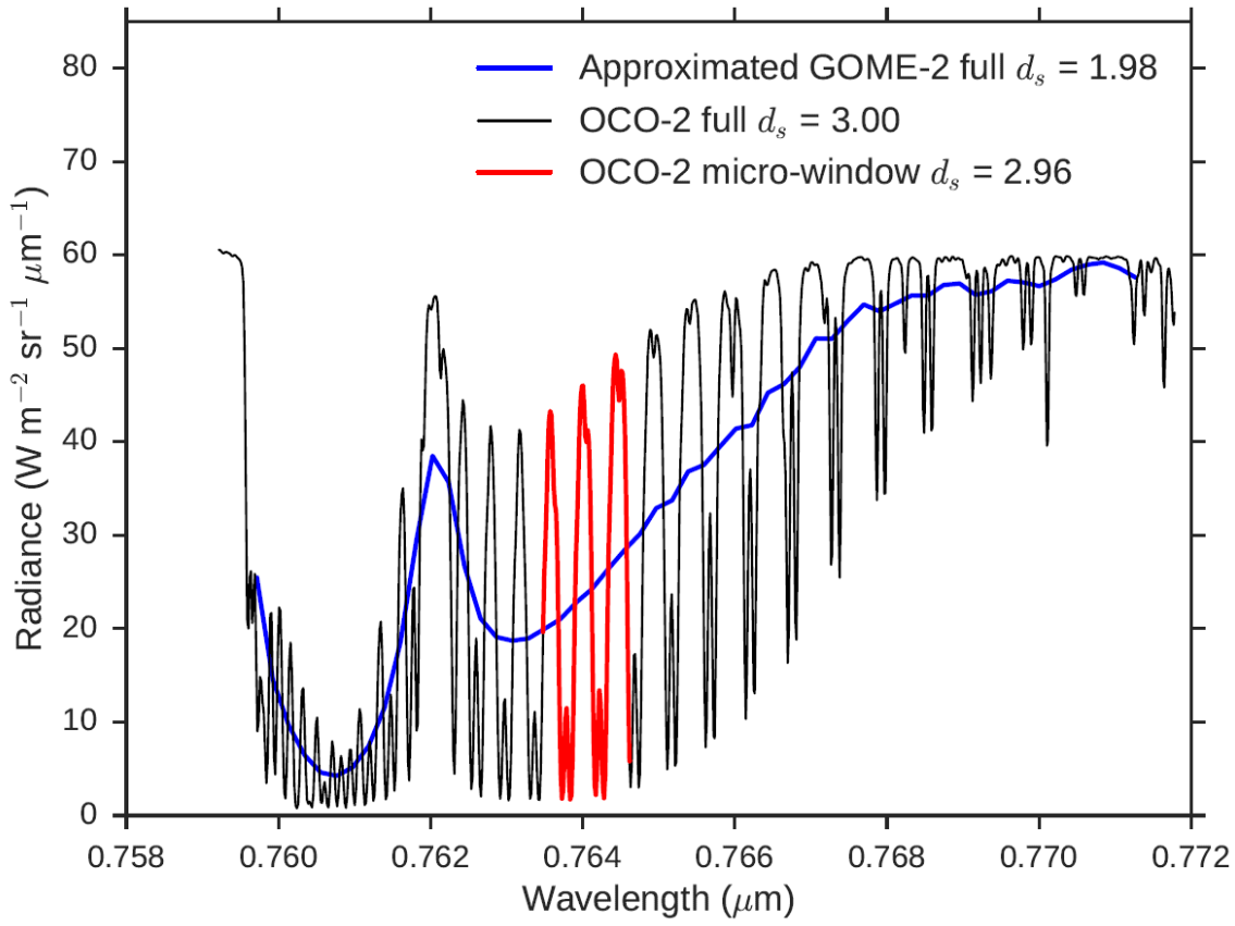
Figure 6 Example simulated cloudy scene A-band spectrum, for a \tau = 10 , P_{top} = 850 hPa cloud in a tropical atmosphere with a solar zenith angle of 45^\circ . The black line shows the full OCO-2 simulated spectrum, the blue line is the black line resampled using approximate GOME-2 instrument line shapes and the red line is the selected 75 channel micro-window for OCO-2 cloud retrievals. The legend also reports the d_s for each spectrum with the GOME-2 instrumental uncertainty based on an SNR of 100 as in previous work (Schuessler et al., 2014).
