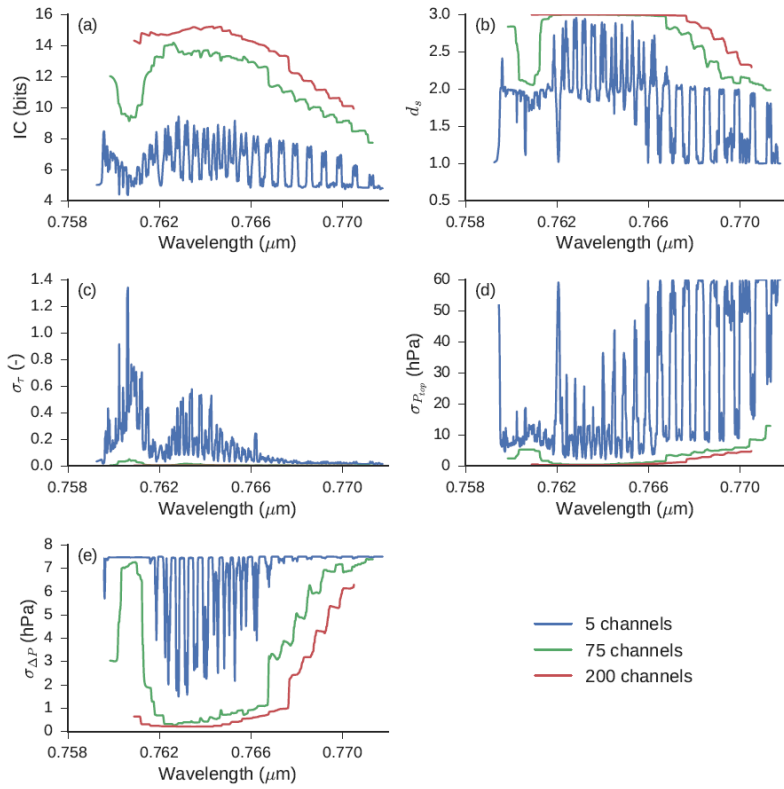
Figure 4 Results of information content analysis for a \tau = 10 and P_{top} = 850 hPa cloud in mean mid-latitude meteorology for OCO-2 sounding position 1. Each line represents the result using a micro-window of difference size, centred on the OCO-2 channel given in the x-axis. Values are as follows: (a) information content in bits, (b) degrees of freedom for signal, (c—e) square root of diagonal elements of posterior state covariance matrix, (c) cloud optical depth, (d) cloud-top pressure and (e) cloud pressure thickness.
