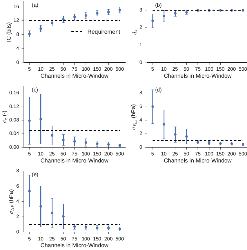
Figure 5 Range of performance for best-located micro-window of each size. The point represents the central value and the lines the full range of the 216 outputs covering each sounding position, meteorology and cloud case. Note that the x-axis is non-linear. (a) Information content in bits, (b) degrees of freedom for signal, (c—e) square root of diagonal covariance matrix elements: (c) cloud optical depth, (d) cloud-top pressure and (e) cloud pressure thickness. Dashed lines represent selected retrieval requirements.
