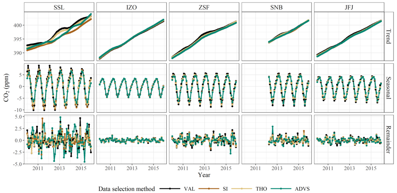
Figure 4: STL decomposition results from VAL (black), SI-selected (brown), THO-selected (yellow), and ADMS ADVS -selected (green) data-sets at five GAW stations.
