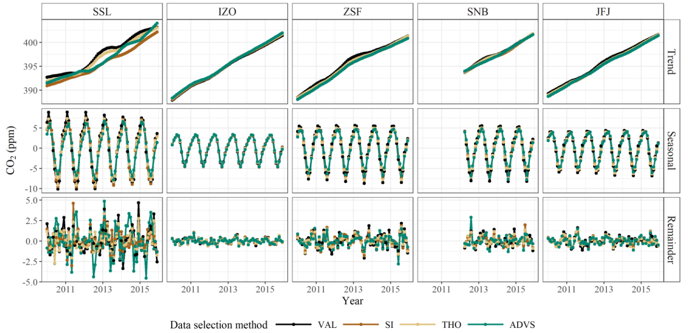
Figure 4: STL decomposition results from VAL (black), SI-selected (brown), THO-selected (yellow), and ADMY ADVS -selected (green) data-sets at five GAW stations.
