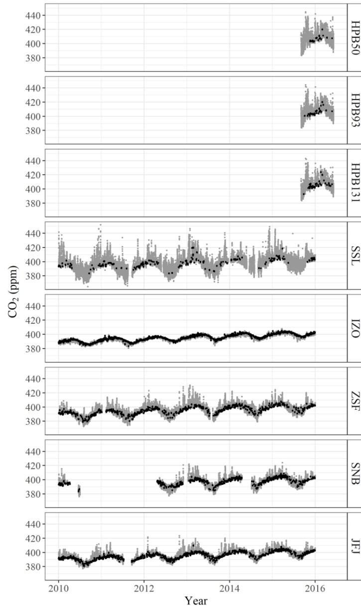
Figure 3: Time series plots of validated CO 2 datasets (gray), and selected data-sets by ADXS ADMV (black) at six GAW stations.
