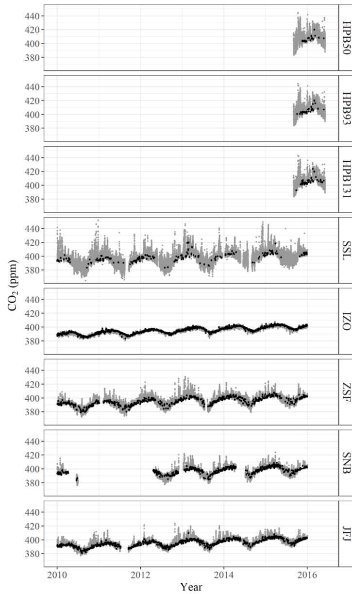
Figure 3: Time series plots of validated CO 2 datasets (gray), and selected data-sets by ADMV (black) at six GAW stations.
