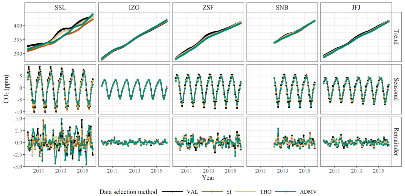
Figure 4: STL decomposition results from VAL (black), SI-selected (brown), THO-selected (yellow), and ADMV - selected (green) data-sets at five GAW stations.
