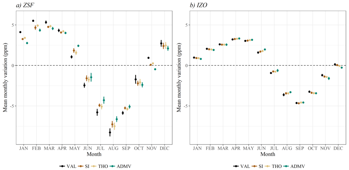
Figure 5: Mean monthly variation of the seasonal component decomposed by STL at a) ZSF and b) IZO over the whole period. For better visualization of the results of selection methods, dots have been separated horizontally equidistantly. The 95% confidence intervals are shown as error bars.
