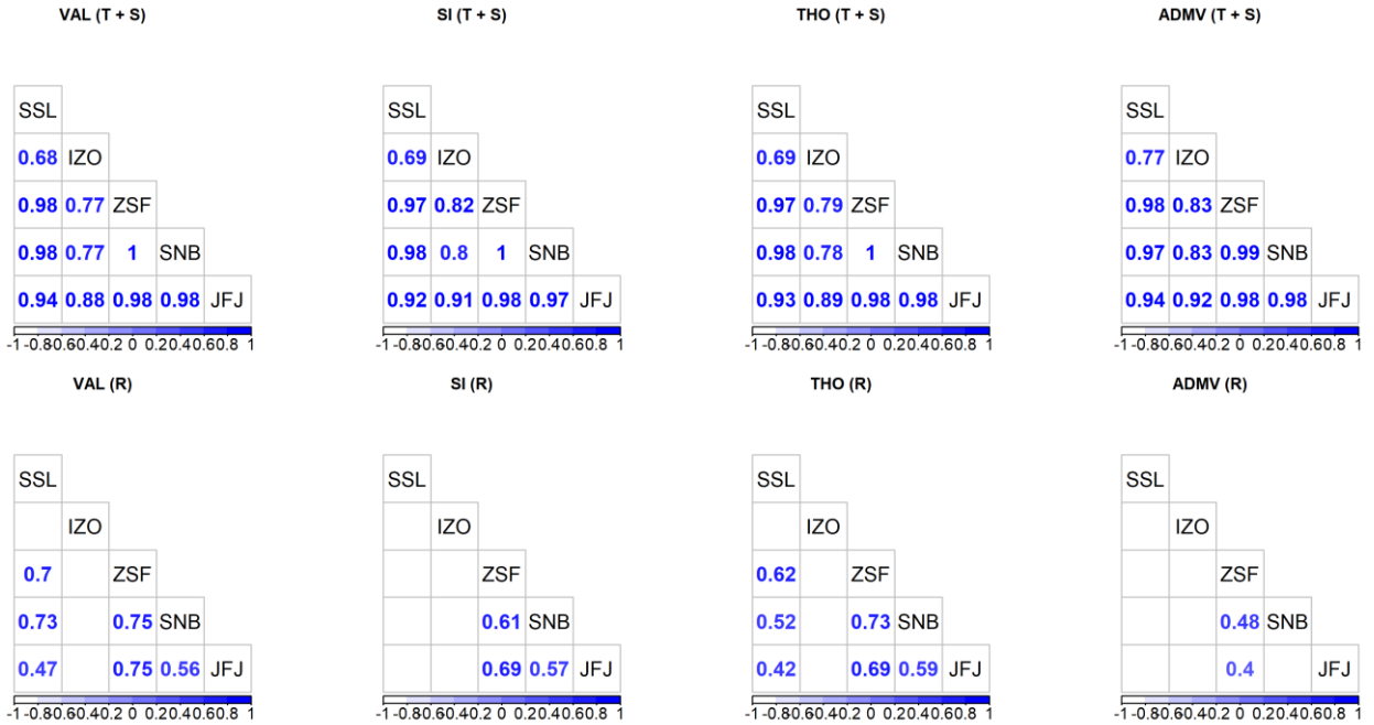
Figure 6: Pearson's correlation matrices of combinations of trend (T) and seasonal (S) components (upper panel), and only remainder (R) components (lower panel) at stations SSL , IZO , ZSF , SNB , and JFJ by different selection methods, as indicated on the top. The color scale reflects the strength of correlation. Correlations with no significant coefficient at the 0.05 confidence level were left blank.
