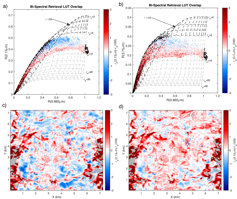
5 Figure 7: Panel (a) and (b) depict the standard bispectral LUT (light gray dashed lines) for both SWIR bands with the scattered reflectance points for the ATEX polluted LES case plotted overtop. The scatterplot is colored by the bias between the bispectral retrieval and the physical reference ( r_c(\text{bispectral}) - r_c(\text{VW}) ), which is also shown below as a spatial variability map. Note that some points are colored in black to indicate retrieval failure due to falling outside the LUT space. In addition to the standard LUT, an extended LUT including droplet sizes from 2-4 \mu\text{m} is included (black dashed lines), revealing an overlapping region of the two LUT for smaller \tau referred to as the “multiple solution space”.
