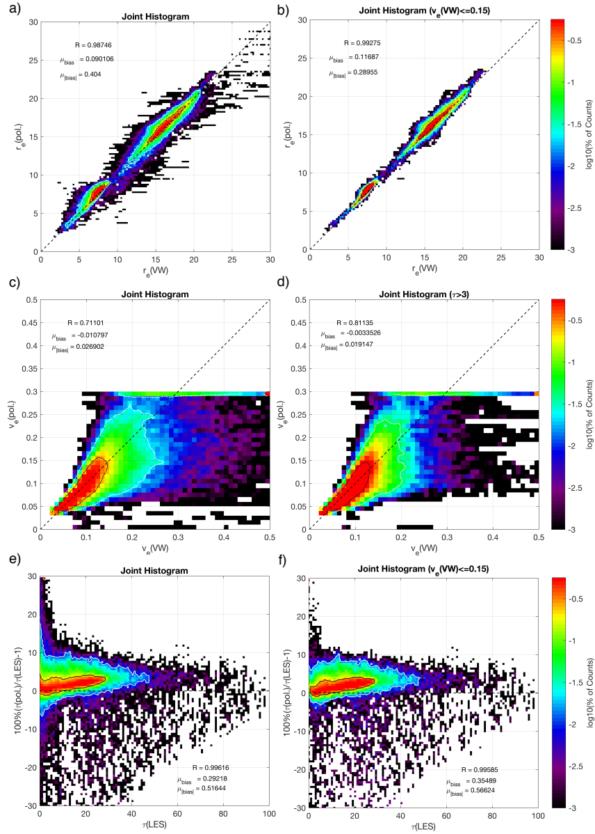
5 Figure 4: Joint histogram regressions of r_e , v_e , and \tau in all LES cases comparing the polarimetric retrievals to the LES cloud microphysical properties. Panel (a) depicts the regression of the polarimetric r_e(\text{pol}) retrieval against the physical analogue r_e(\text{VW}) , while panel (b) is sub-selection of the same regression for low v_e . Panel (c) depicts the regression of the polarimetric v_e(\text{pol}) retrieval against the physical analogue v_e(\text{VW}) , while panel (d) is a sub-selection of the same regression for thick clouds ( \tau > 3 ). Panel (e) depicts the regression of the polarimetric \tau(\text{pol}) retrieval against the physical analogue \tau(\text{LES}) , while panel (f) is sub-selection of the same regression for low v_e . Note that in each panel the correlation is quantified with a linear correlation coefficient ( R ) and the black and white contours encompass 66% and 95% of the population, respectively.
