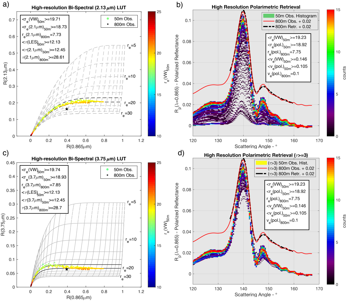
Figure 11: Panels (a) and (c) depict the bispectral LUT's and 50 m reflectances for the 2.13 and 3.75 \mu\text{m} bispectral retrievals respectively for a particularly inhomogeneous 800 m pixel. The scattered points correspond to 50 m reflectances with color corresponding to r_e(VW) , while the black star corresponds to the 800 m reflectance pair (the average of the 50 m data). The polarimetric reflectance distribution histograms in panels (b) and (d) address how the high-resolution (50 m) reflectance distribution influences the polarimetric retrieval at coarse resolution (800m). The two curves (plotted with a 0.02 reflectance shift for clarity) are the 800 m observed reflectance (black dashed curve) and the 800 m retrieval (red solid curve). All of these figures include statistics on the high-resolution averages of physical properties and retrievals along with their coarse resolution counterparts for comparison.
