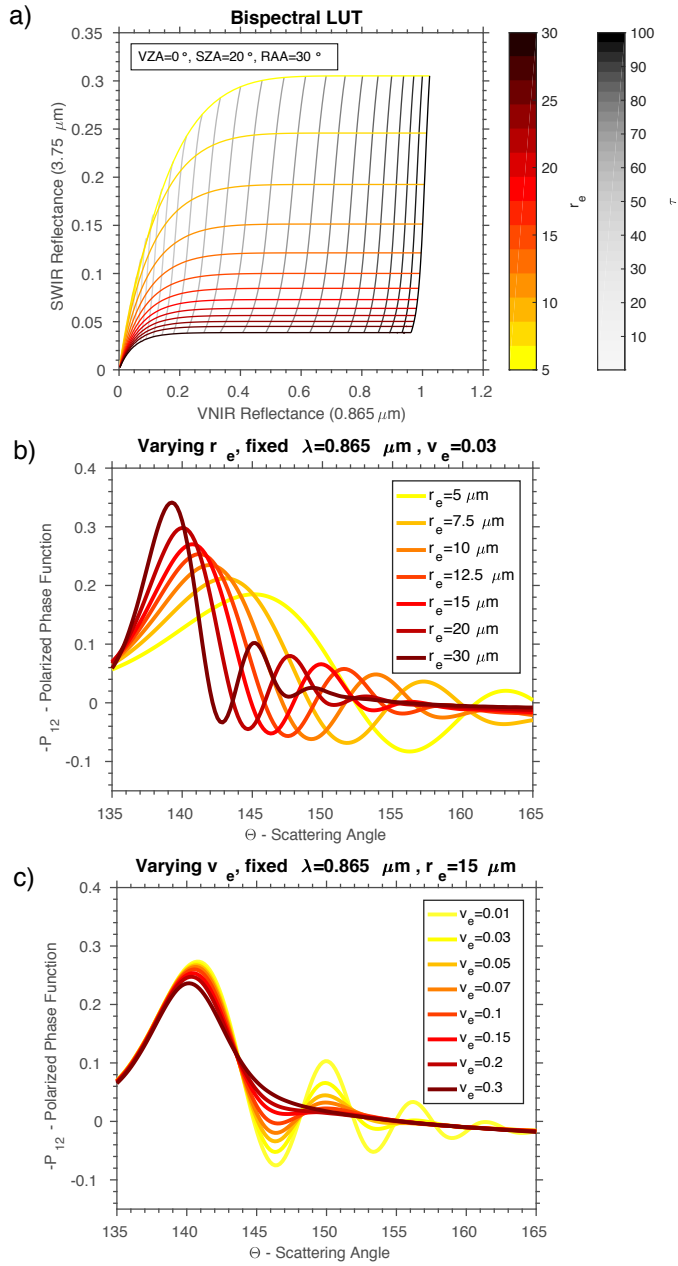
Figure 1: Demonstrations of the microphysical sensitivity of the bispectral and the polarimetric techniques. Panel (a) features the bispectral LUT exhibiting sensitivity to r_e (colored iso-lines), due to absorption in the SWIR/ reflectance. The VNIR reflectances provide sensitivity to optical thickness (gray iso-lines). Panels (b) and (c) demonstrate the sensitivity of polarimetric technique to r_e and v_e respectively. The supernumerary bow peaks of the polarized phase function ( -P_{12} ) shift and become narrower with increasing droplet size ( r_e ), whereas the peaks erode in magnitude for broadened droplet size distributions ( v_e ).
