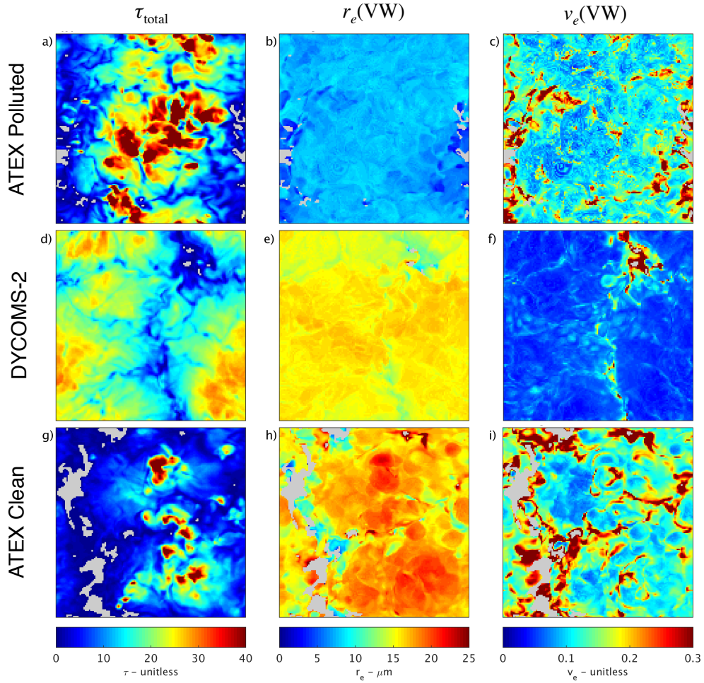
5 Figure 2: The optical and microphysical properties ( \tau , r_e , and v_e ) of the LES cases examined in this study. The panels are arranged such that each LES case appears row-wise and the different properties are appear column-wise. Note that the vertically weighting functions used for the displayed r_e(\text{VW}) and v_e(\text{VW}) correspond to single-scattering assumptions. Cloud-free masking in each of the images appears in gray. Refer to sections 2 and 3 for discussion and definition of each of these properties. Axes labels have been removed to enlarge each map, but the spatial dimensions of each scene are roughly 7 x 7 km (refer to section 3 for the specific resolutions of each LES case.)
