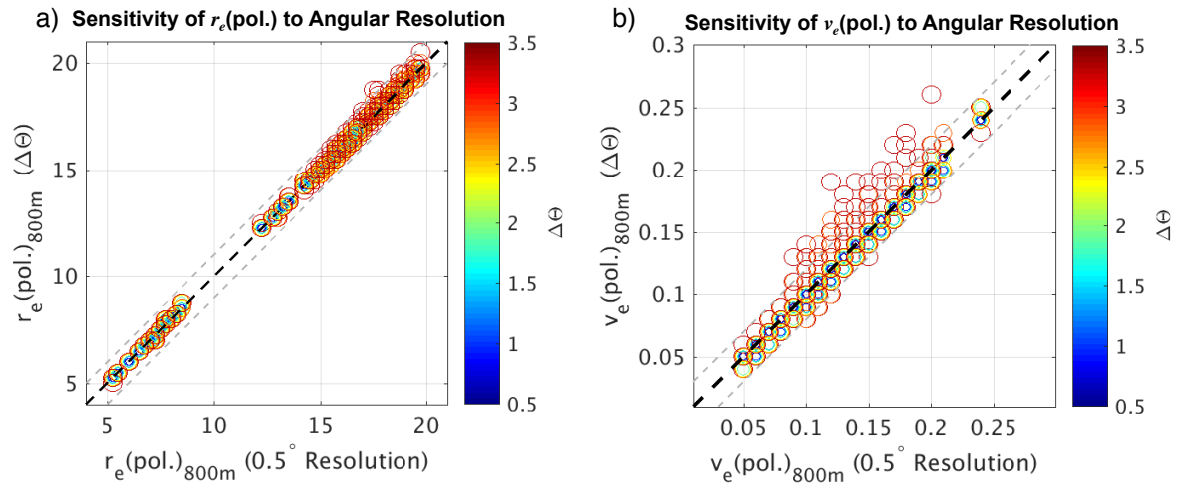
Figure 12: Angular resolution sensitivity experiments examining polarimetric retrievals of r_e (panel a) and v_e (panel b) for all LES scenes at the 800 m spatial resolution. The color and size of scattered points denote the angular resolution of each retrieval. The gray dashed lines denote the \pm 1 step in the LUT space of the polarimetric retrieval.
